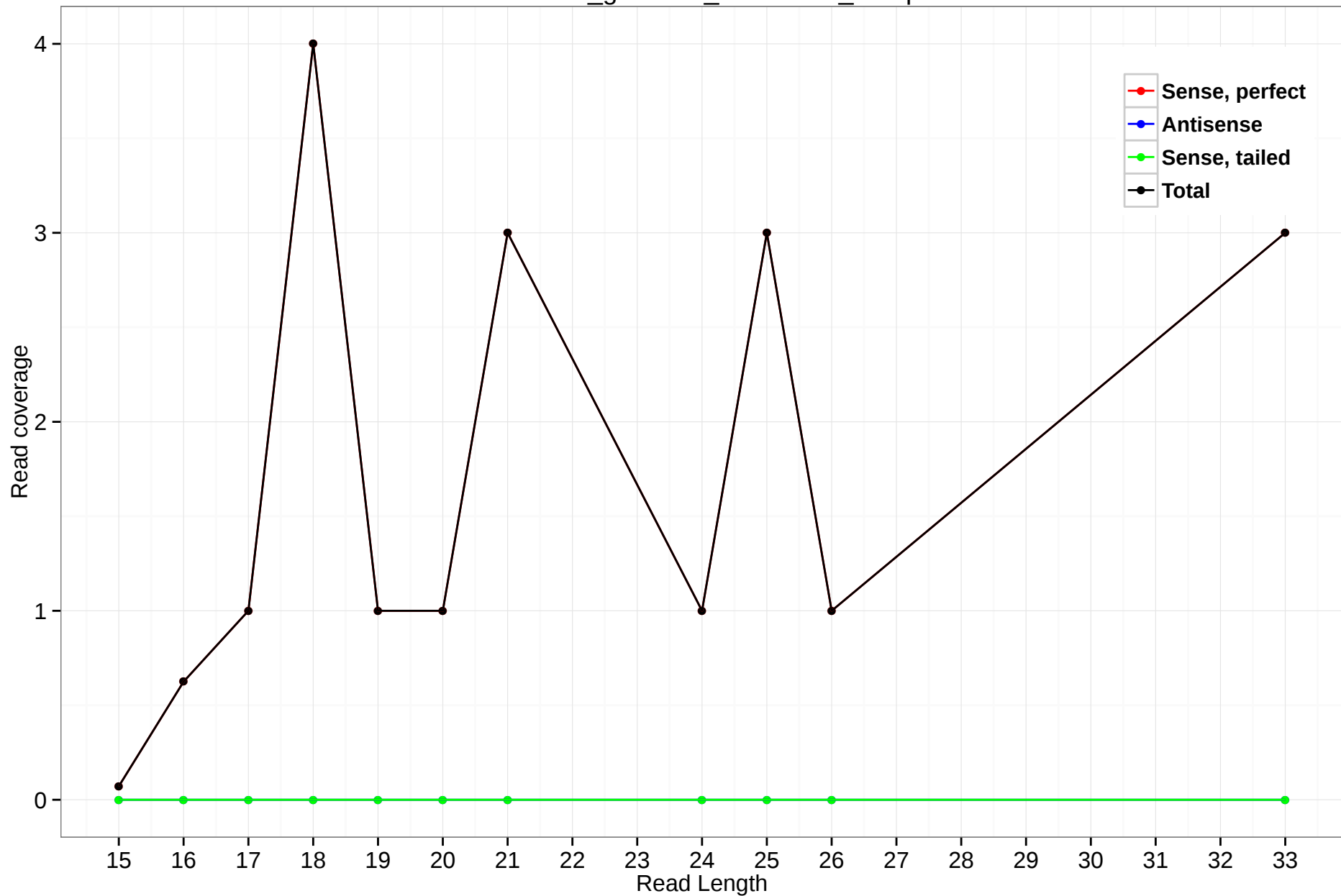
rheMac3_genscan_chr11.827_10.3p
