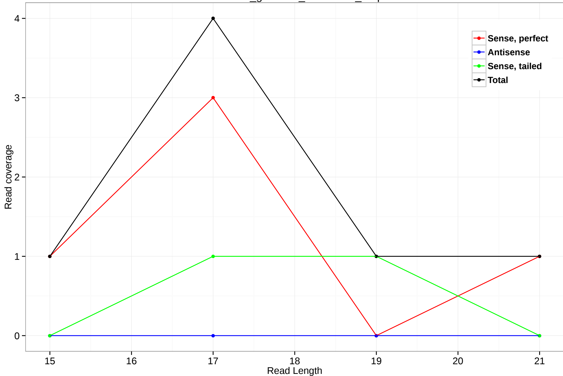
rheMac3_genscan_chr11.809_0.5p
