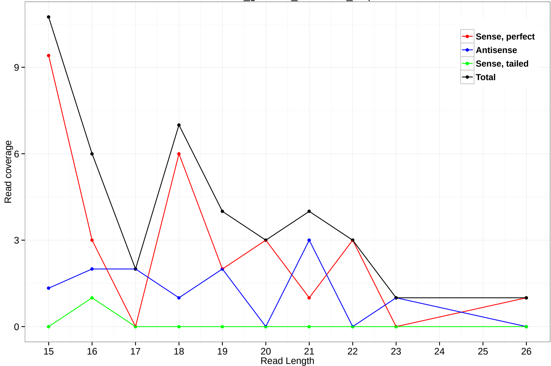
rheMac3_genscan_chr11.770_4.3p
