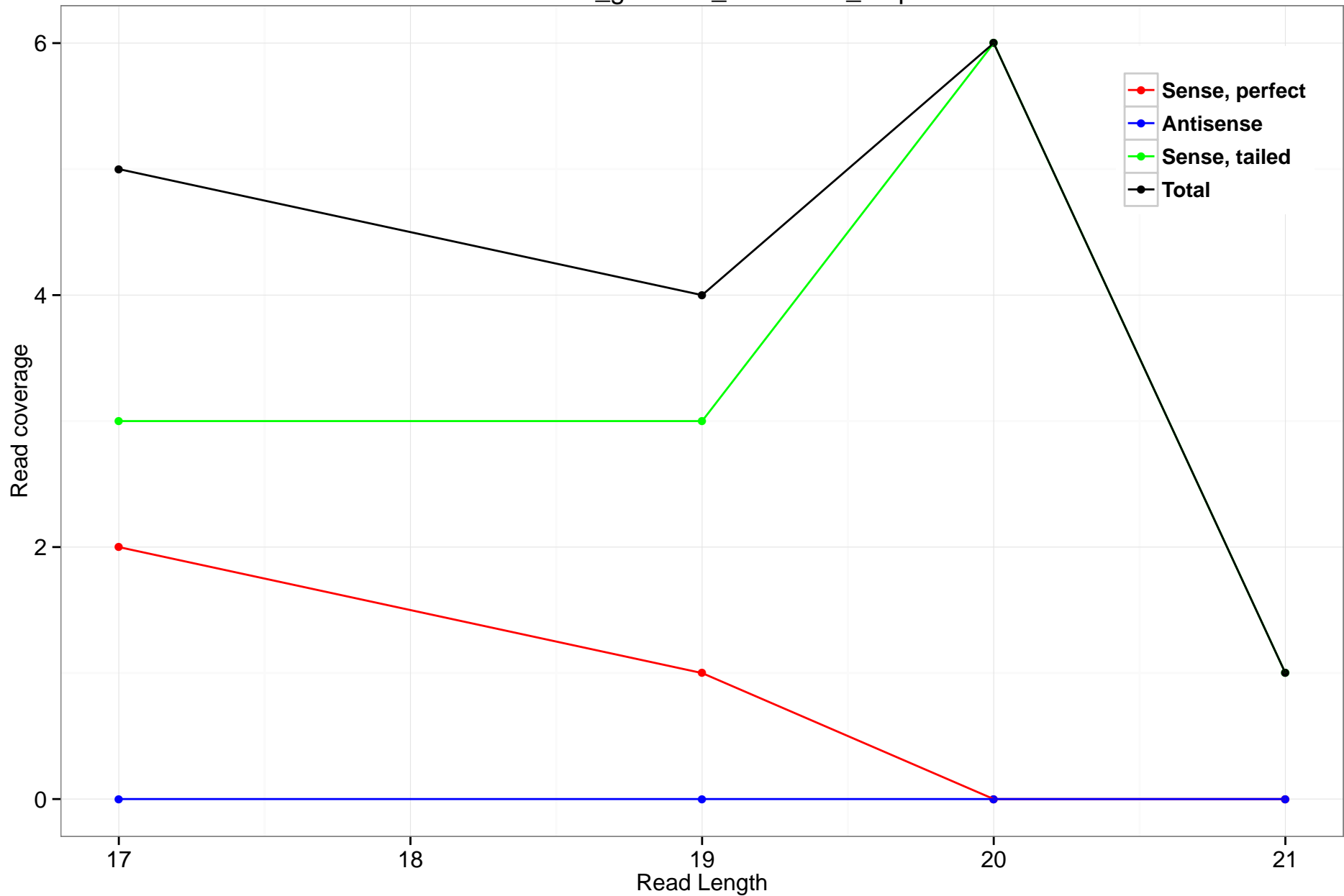
rheMac3_genscan_chr11.769_1.5p
