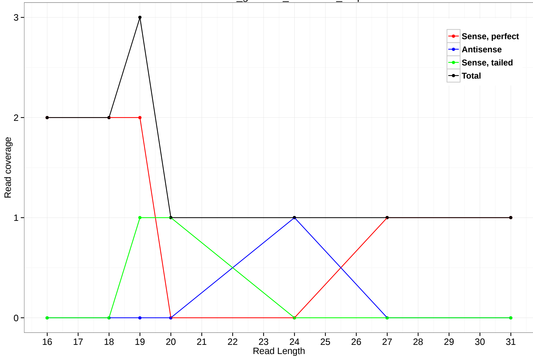
rheMac3_genscan_chr11.767_1.5p
