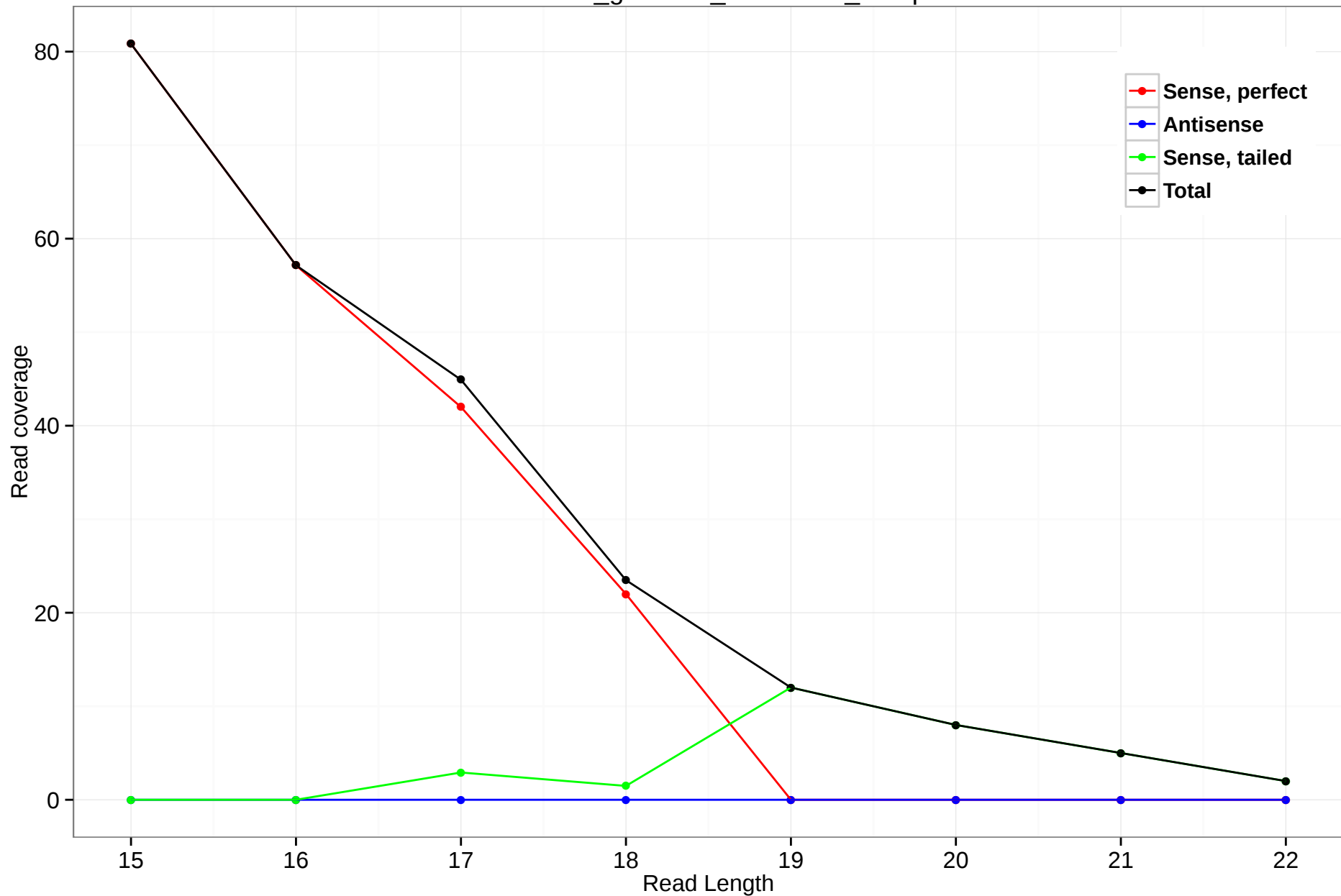
rheMac3_genscan_chr11.695_12.3p
