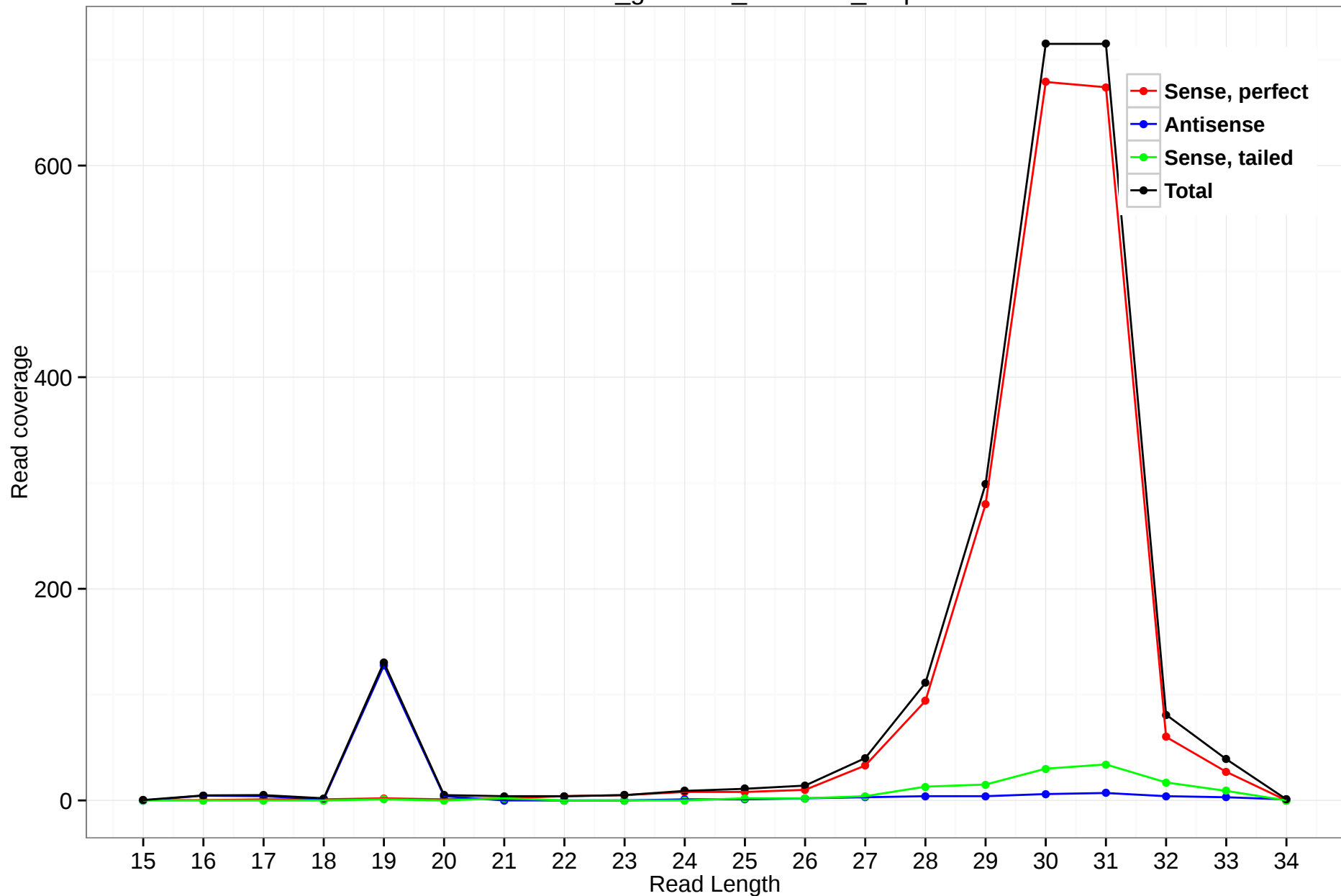
rheMac3_genscan_chr11.67_0.3p
