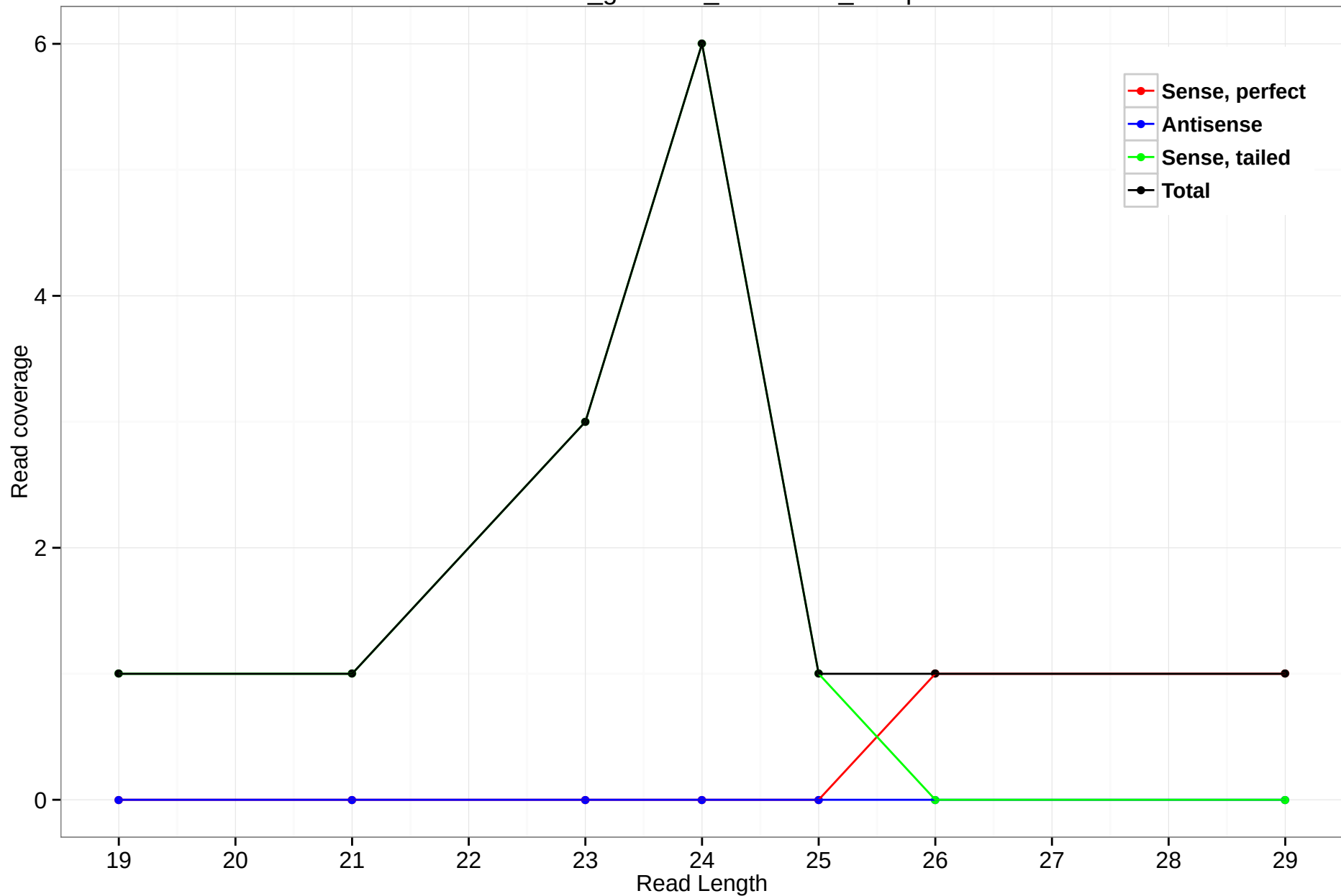
rheMac3_genscan_chr11.659_22.3p
