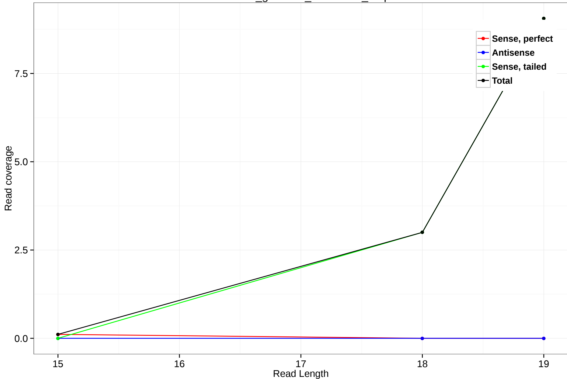
rheMac3_genscan_chr11.642_2.3p
