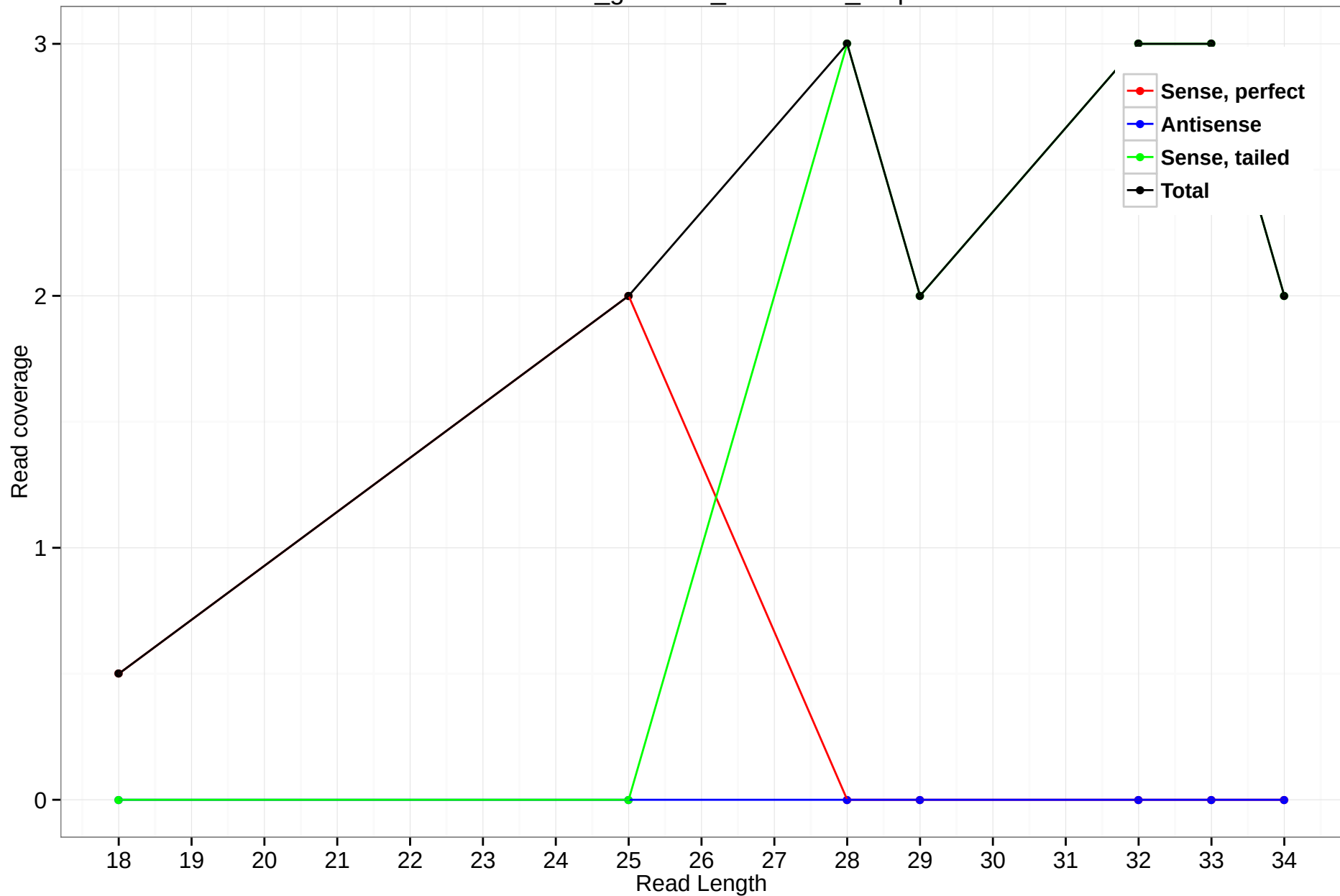
rheMac3_genscan_chr11.637_3.3p
