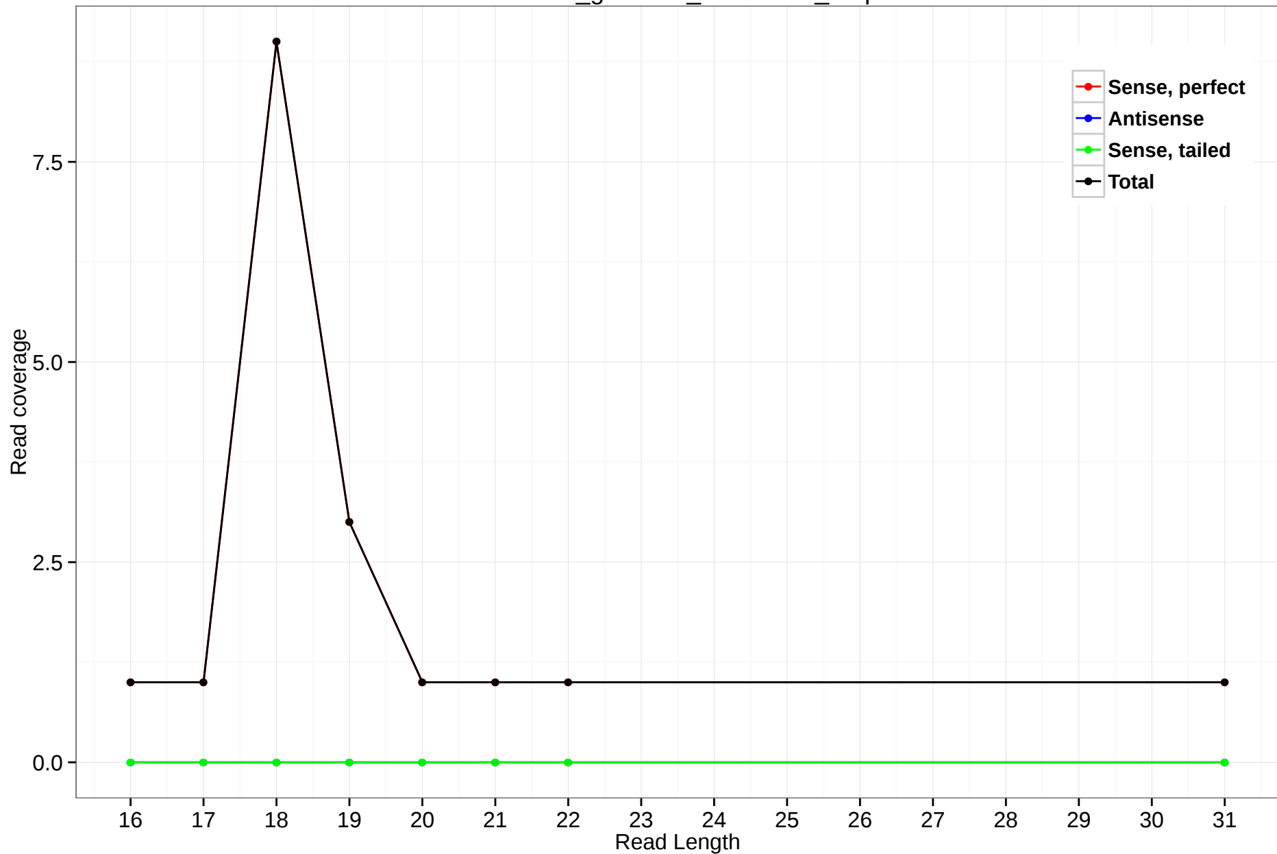
rheMac3_genscan_chr11.637_2.5p
