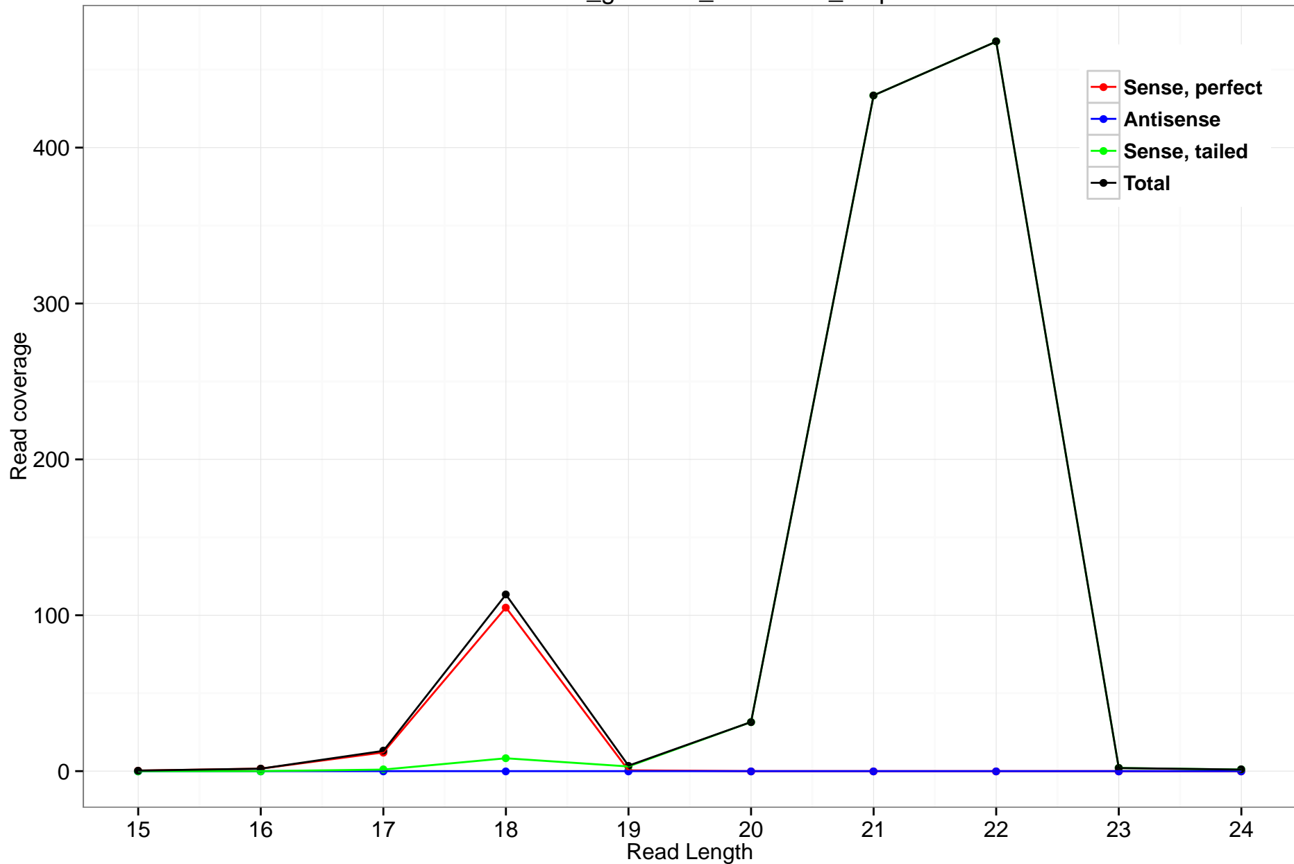
rheMac3_genscan_chr11.634_0.5p
