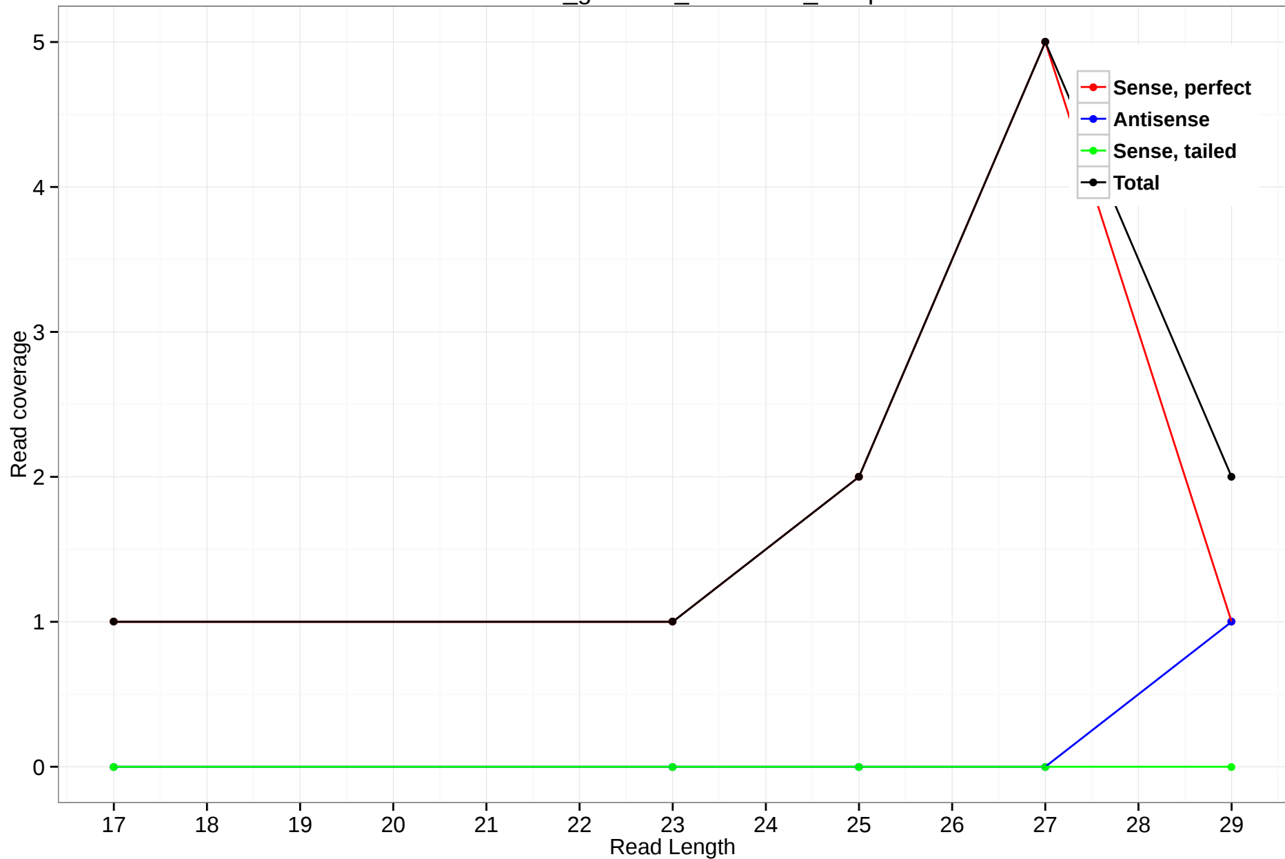
rheMac3_genscan_chr11.627_23.3p
