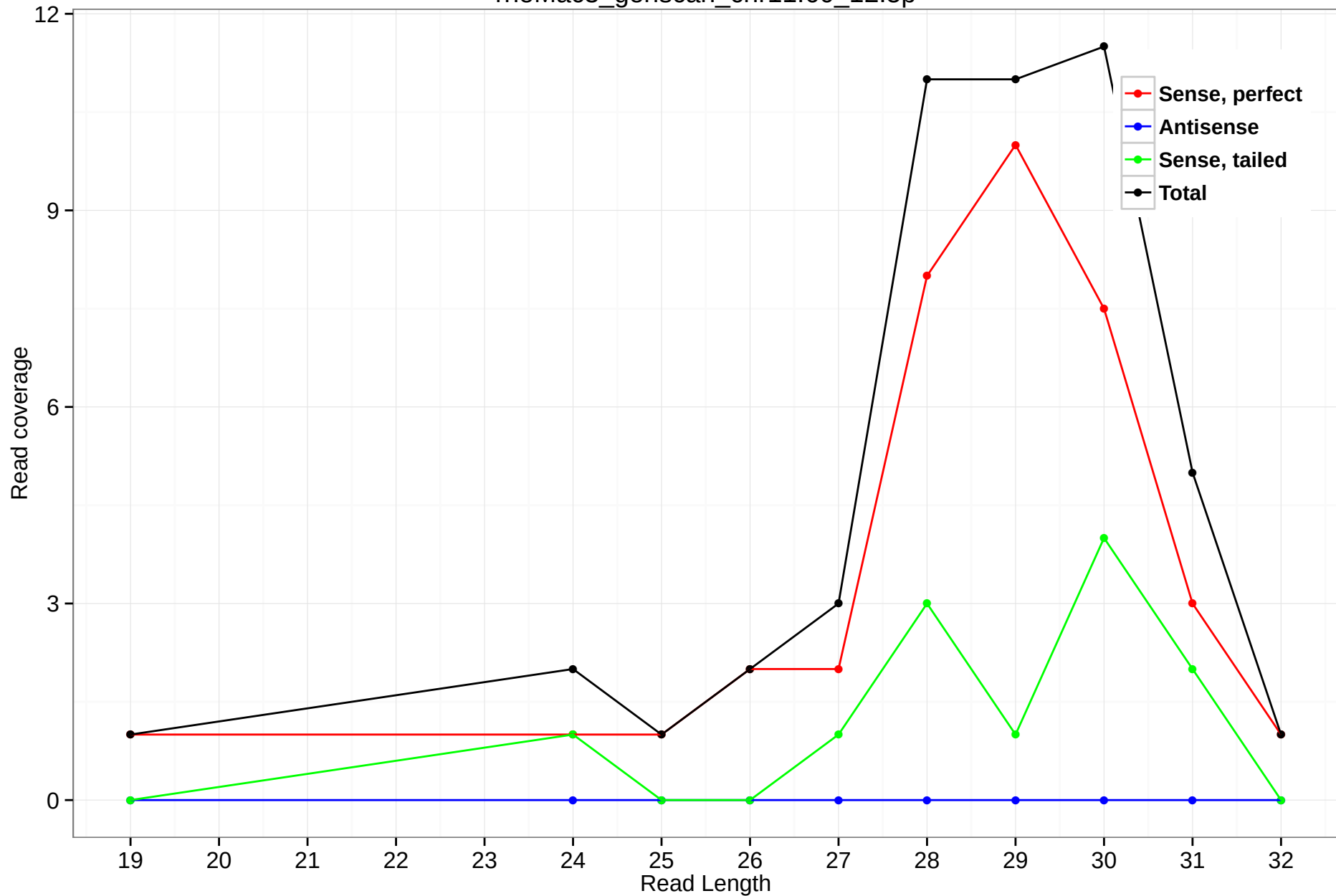
rheMac3_genscan_chr11.60_12.5p
