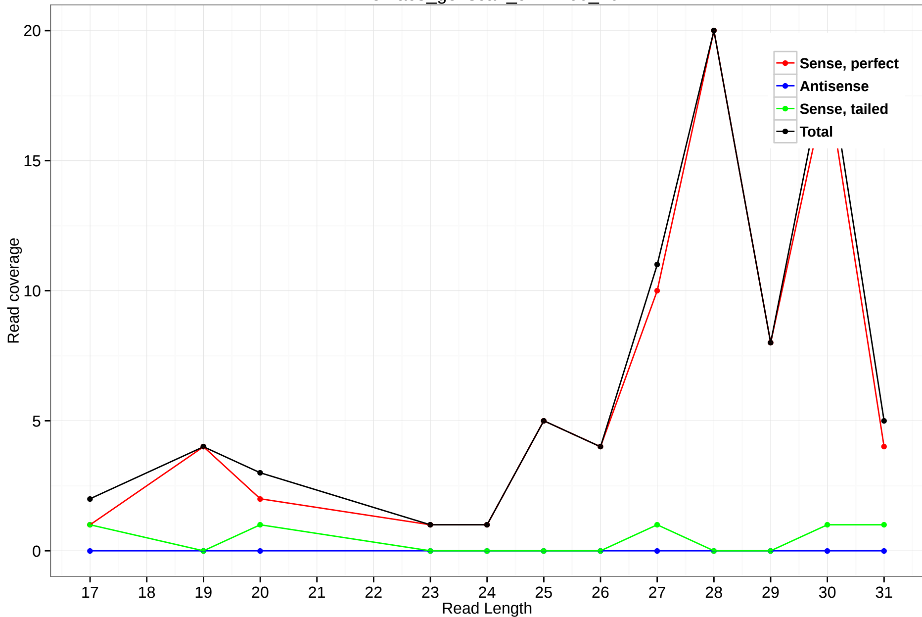
rheMac3_genscan_chr11.60_10
