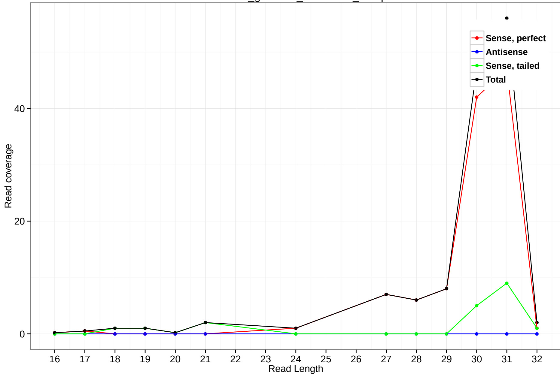
rheMac3_genscan_chr11.608_12.5p
