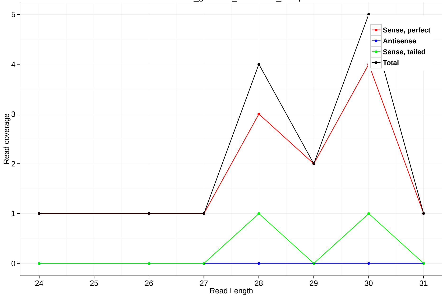
rheMac3_genscan_chr11.608_11.5p
