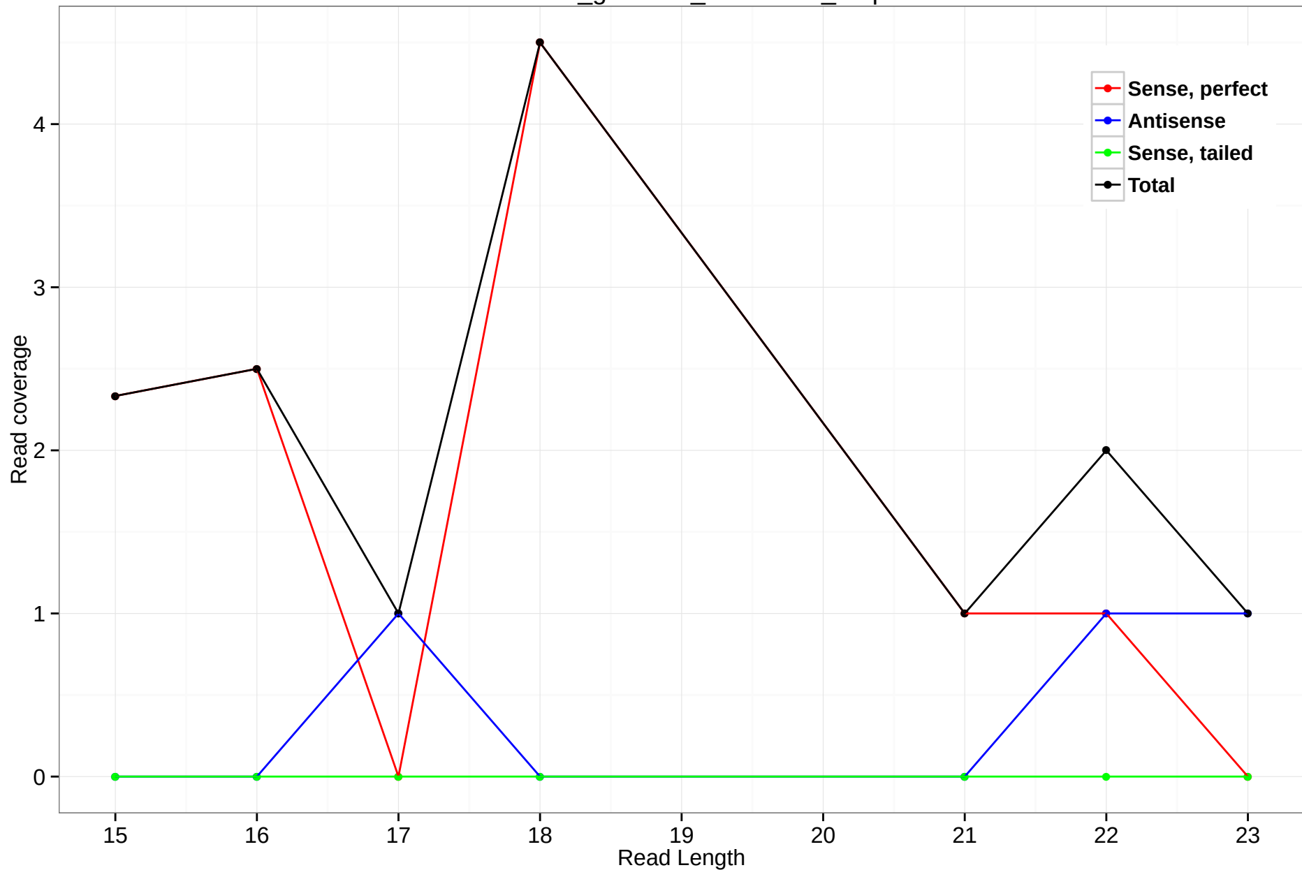
rheMac3_genscan_chr11.544_5.5p
