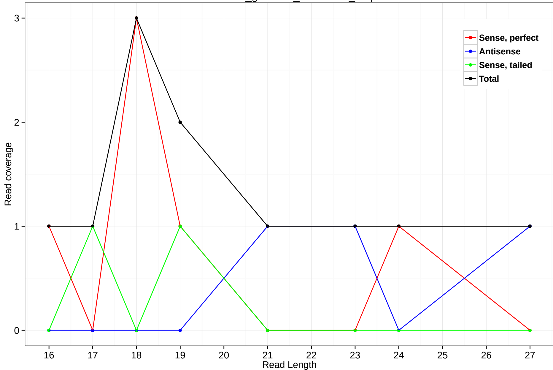
rheMac3_genscan_chr11.544_2.5p
