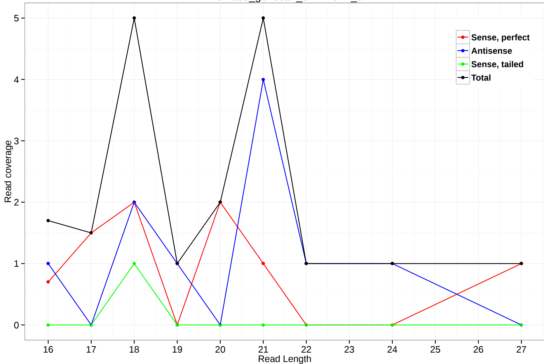
rheMac3_genscan_chr11.542_5
