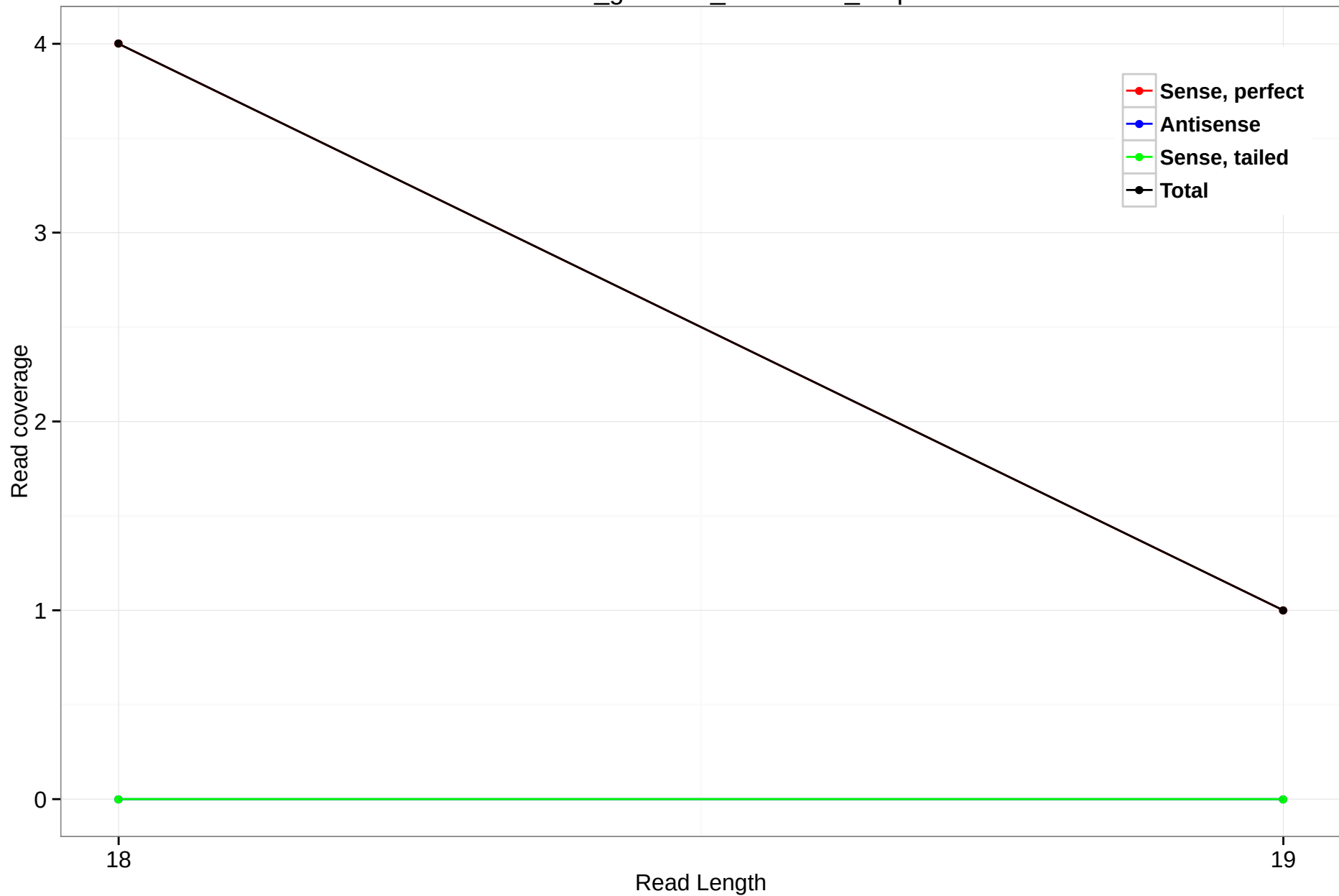
rheMac3_genscan_chr11.513_0.3p
