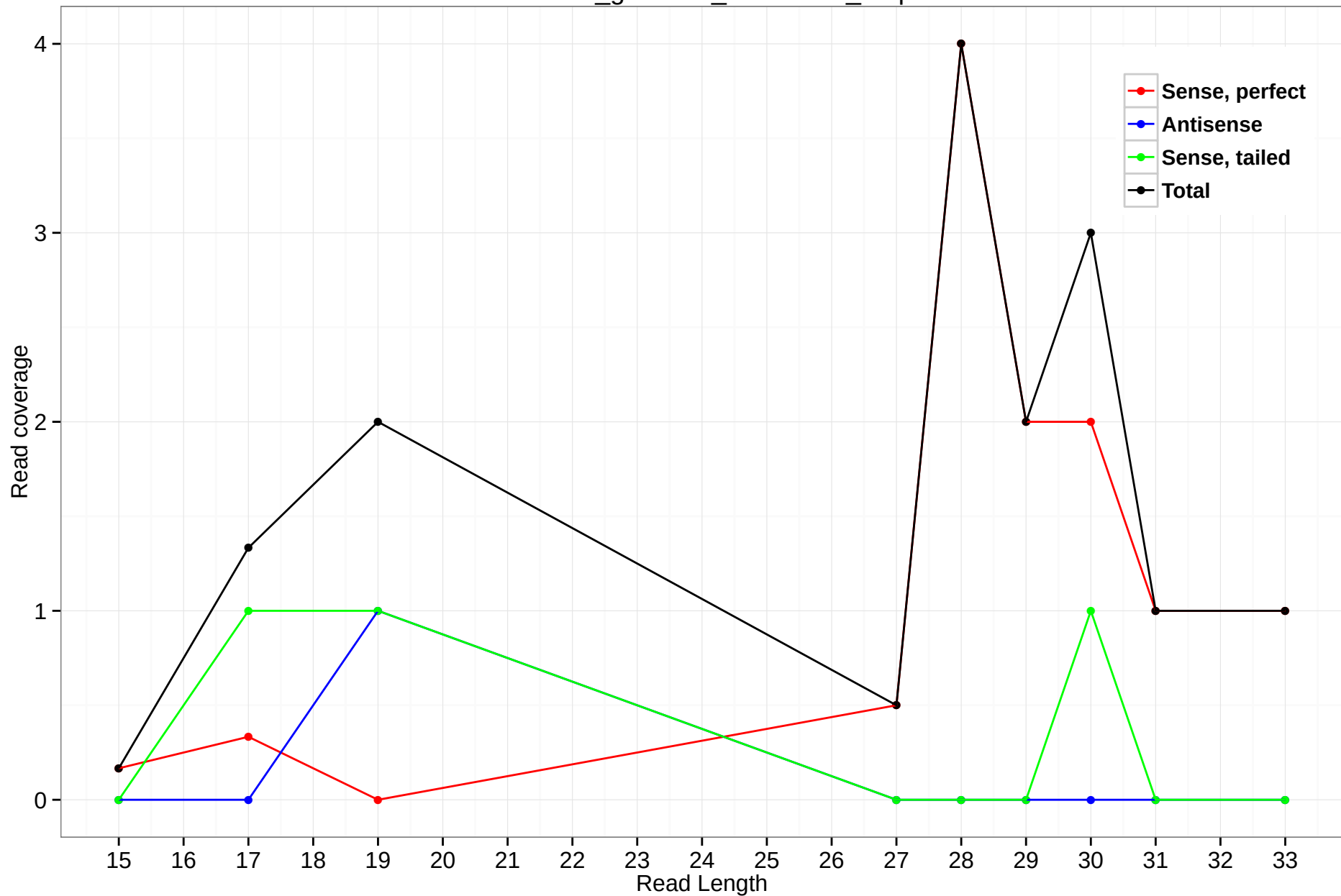
rheMac3_genscan_chr11.437_7.3p
