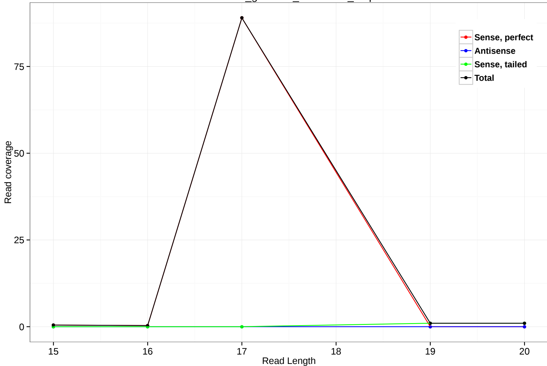
rheMac3_genscan_chr11.350_3.5p
