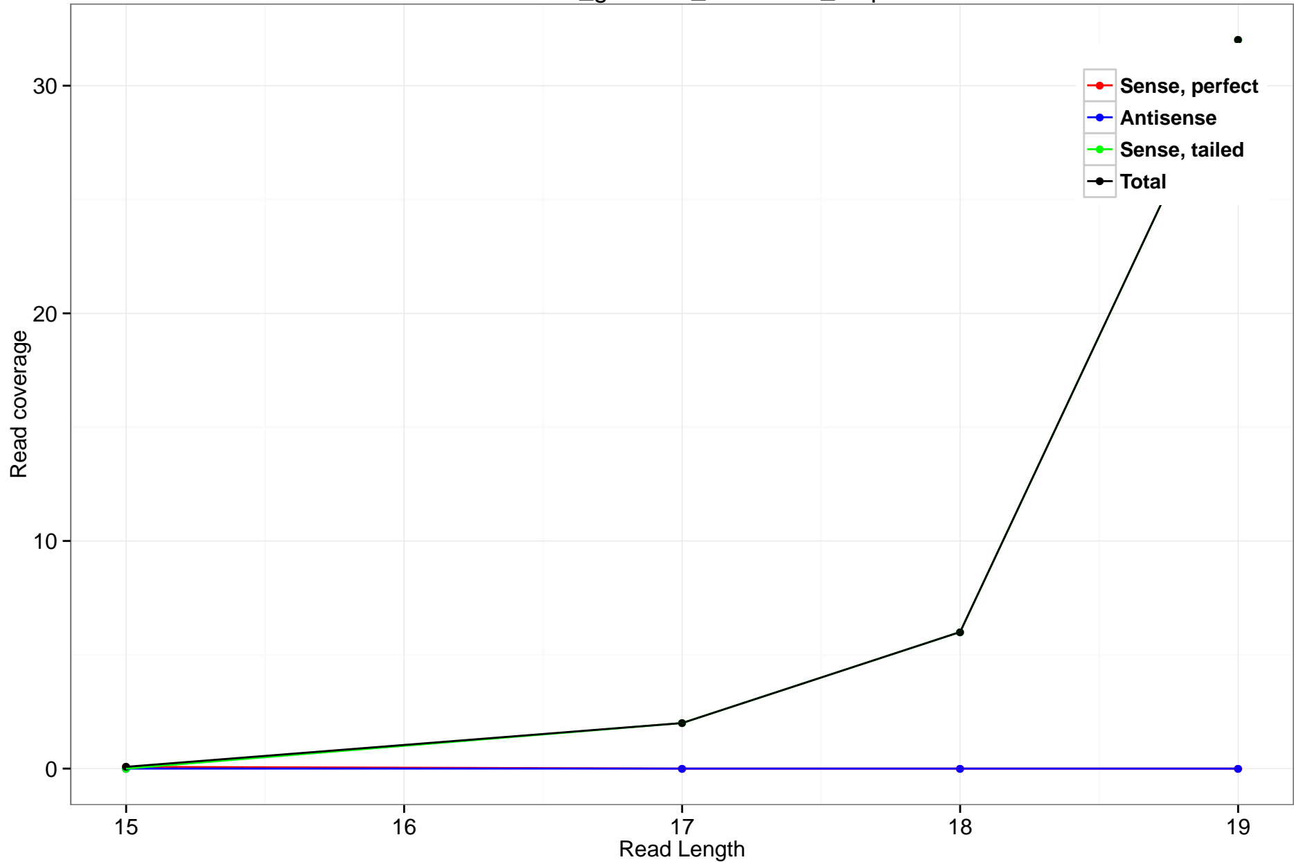
rheMac3_genscan_chr11.338_0.5p
