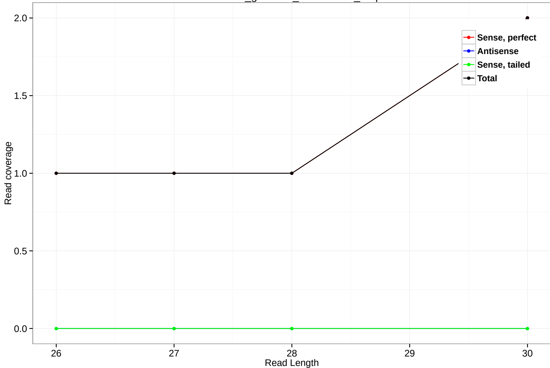
rheMac3_genscan_chr11.2535_2.5p
