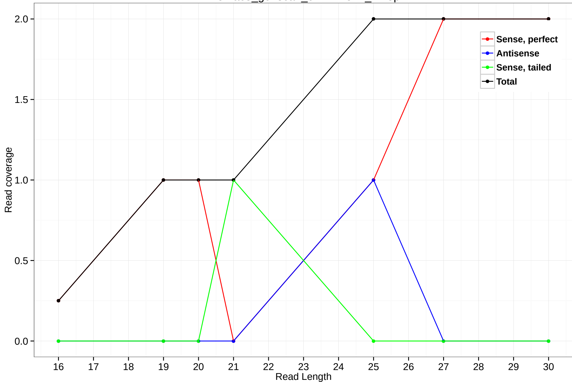
rheMac3_genscan_chr11.2517_42.5p
