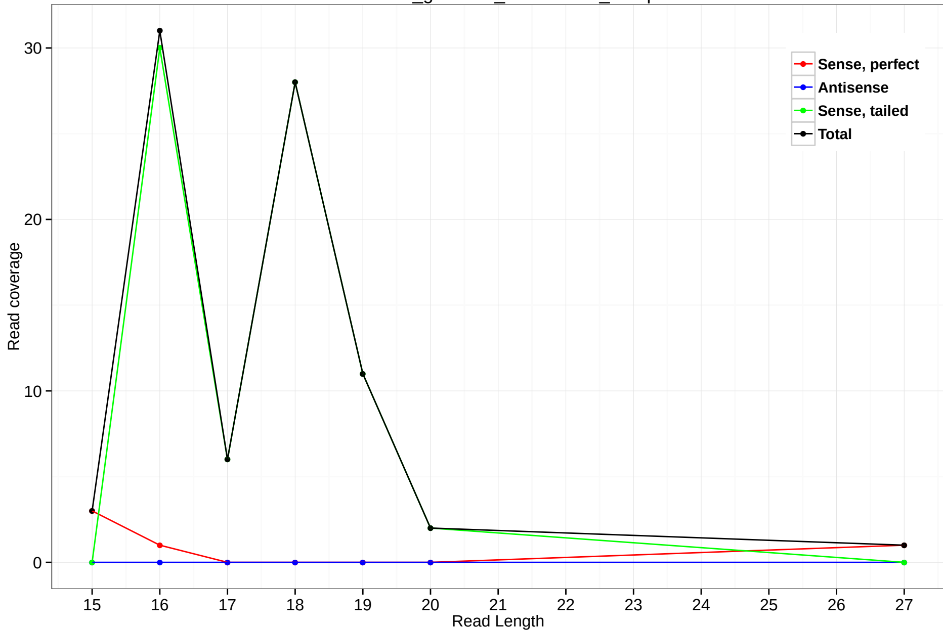
rheMac3_genscan_chr11.2517_30.5p
