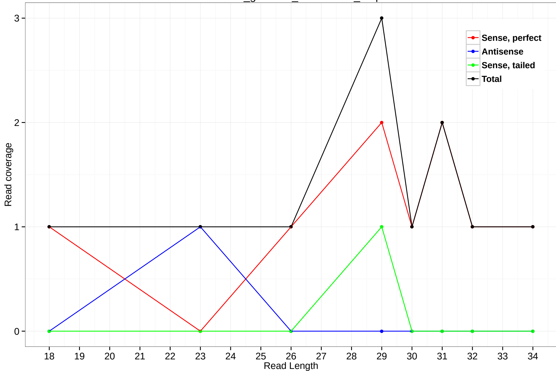
rheMac3_genscan_chr11.2502_0.5p
