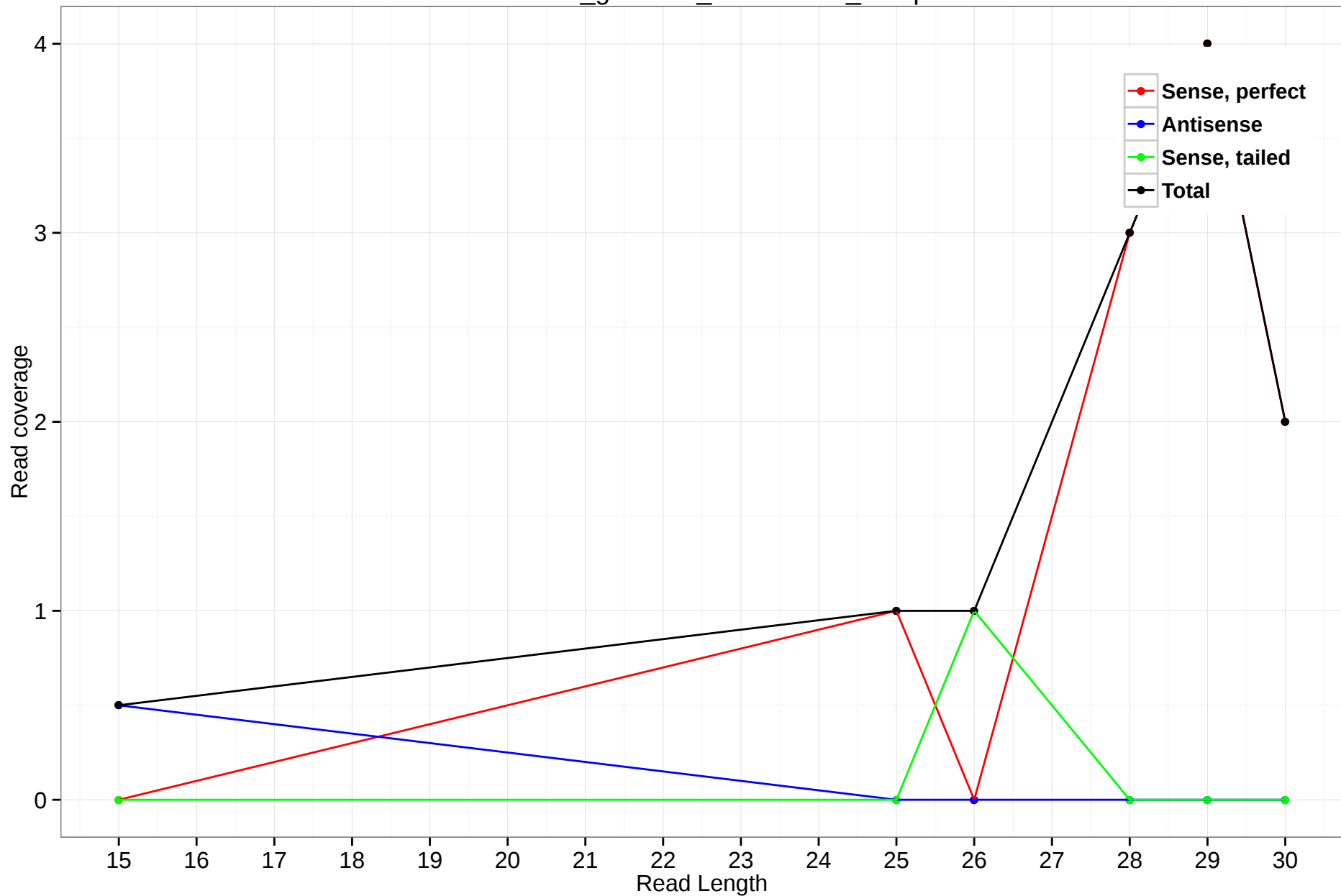
rheMac3_genscan_chr11.2501_53.3p
