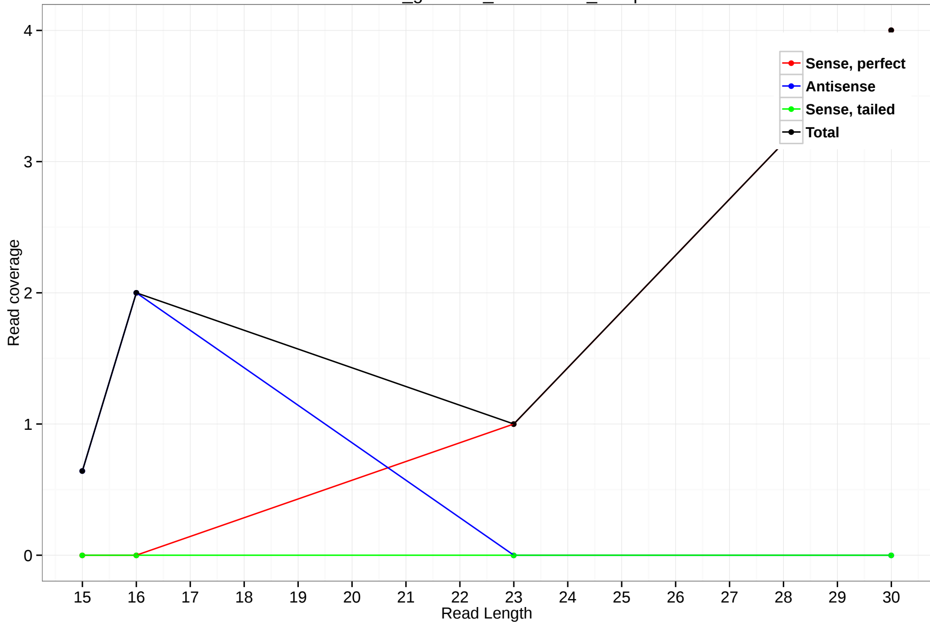
rheMac3_genscan_chr11.2501_52.3p
