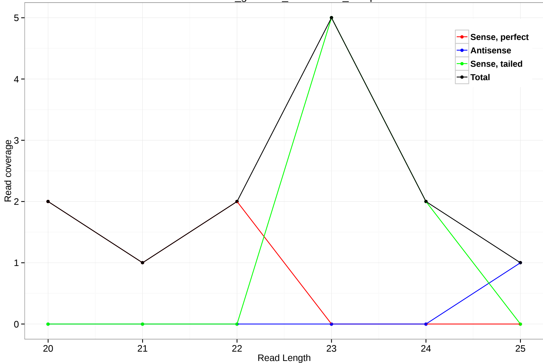
rheMac3_genscan_chr11.2499_22.3p
