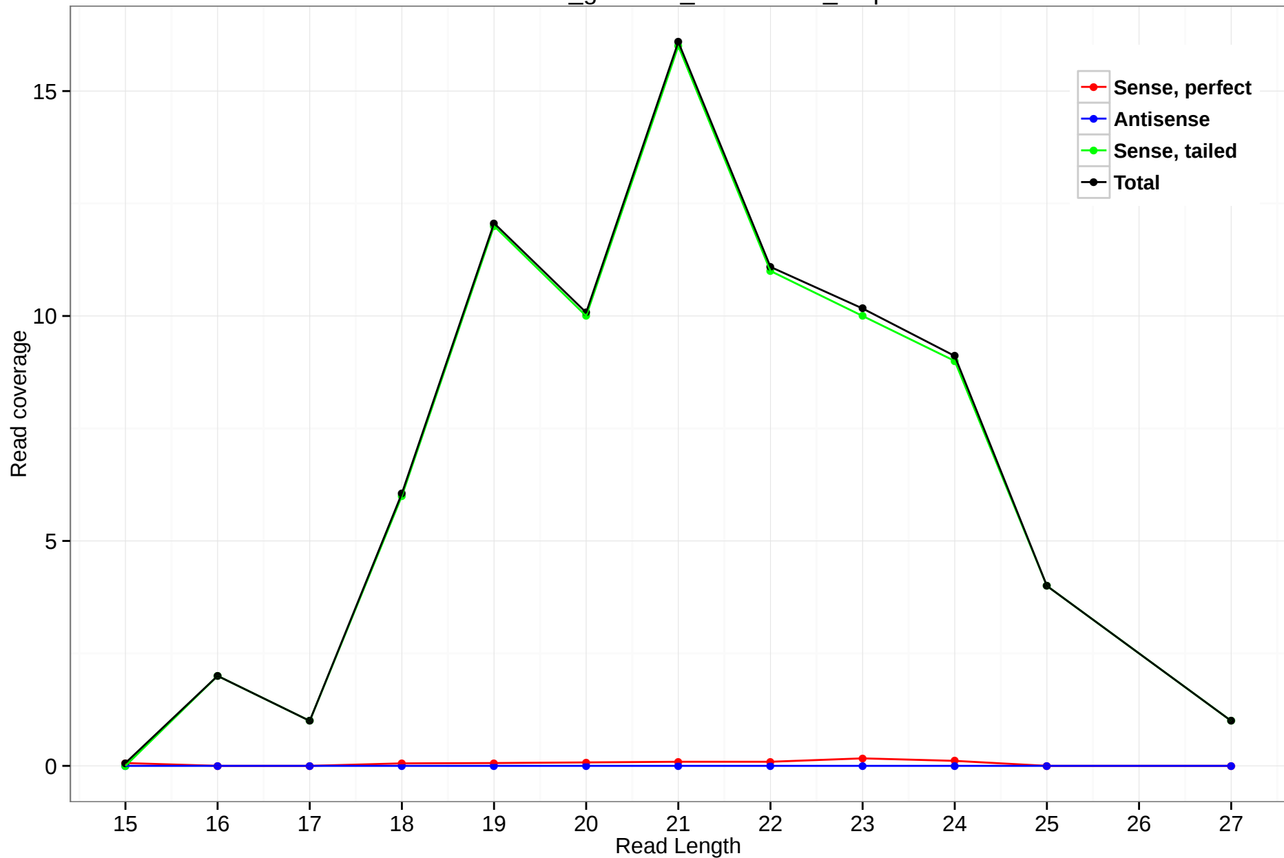
rheMac3_genscan_chr11.2498_2.5p
