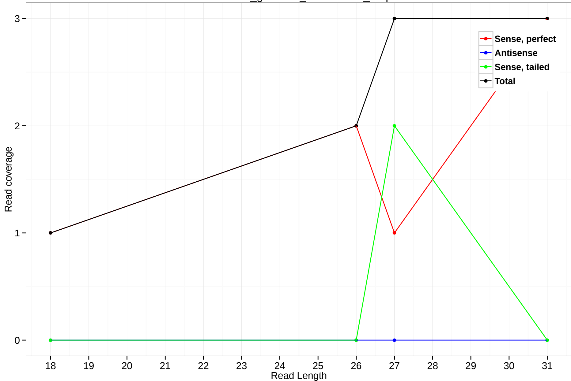
rheMac3_genscan_chr11.2459_6.5p
