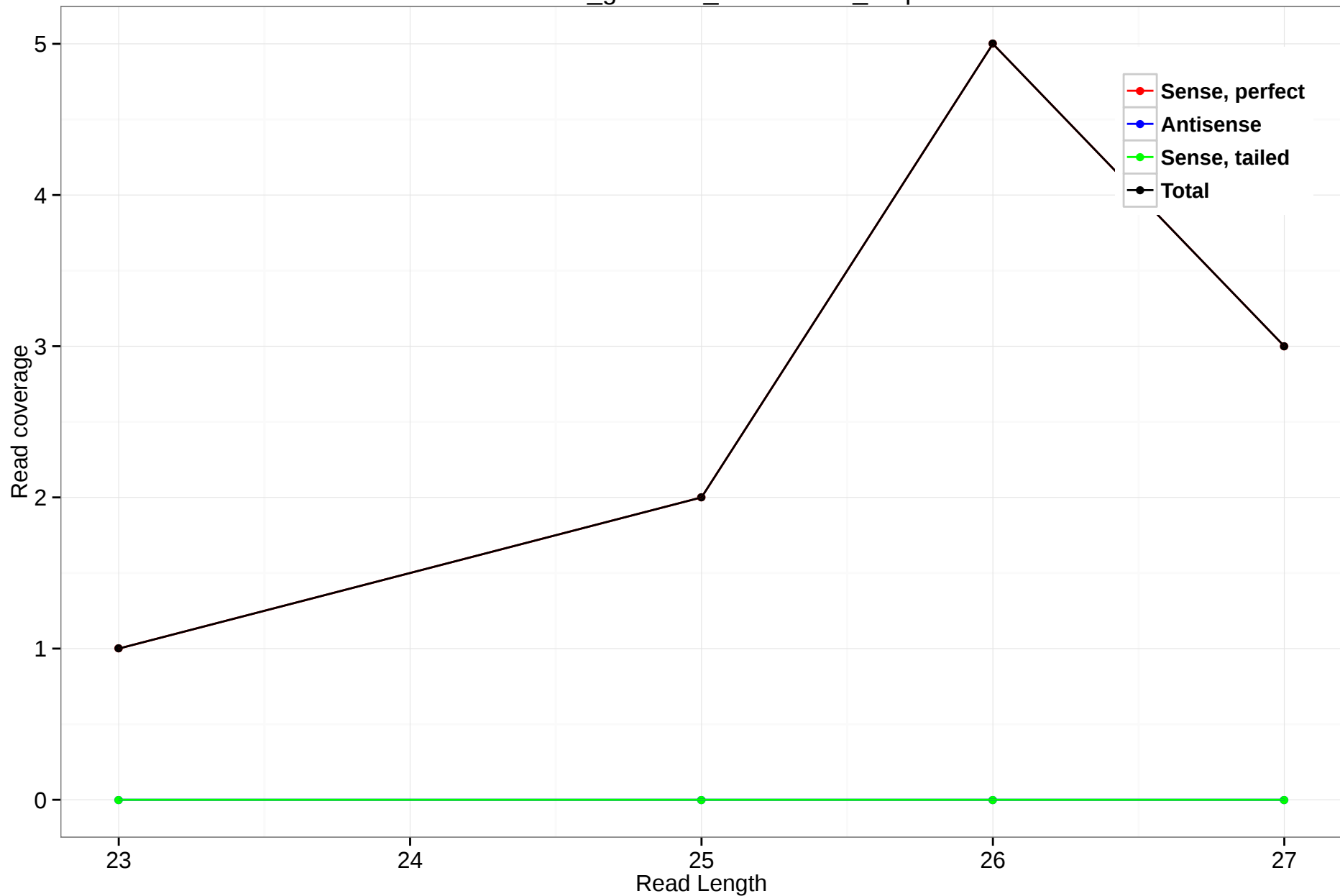
rheMac3_genscan_chr11.2435_2.5p
