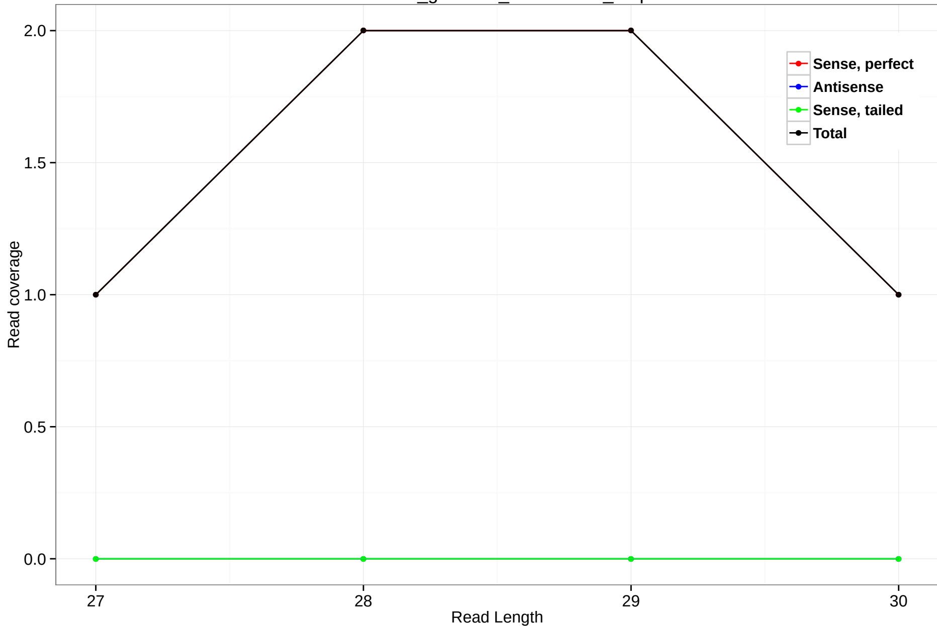
rheMac3_genscan_chr11.2307_5.5p
