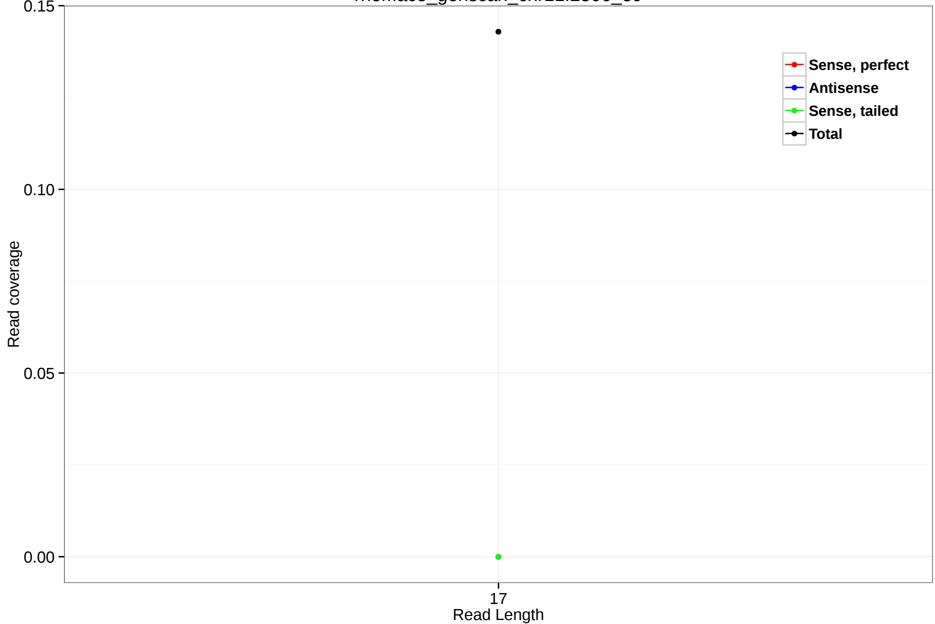
rheMac3_genscan_chr11.2306_39
