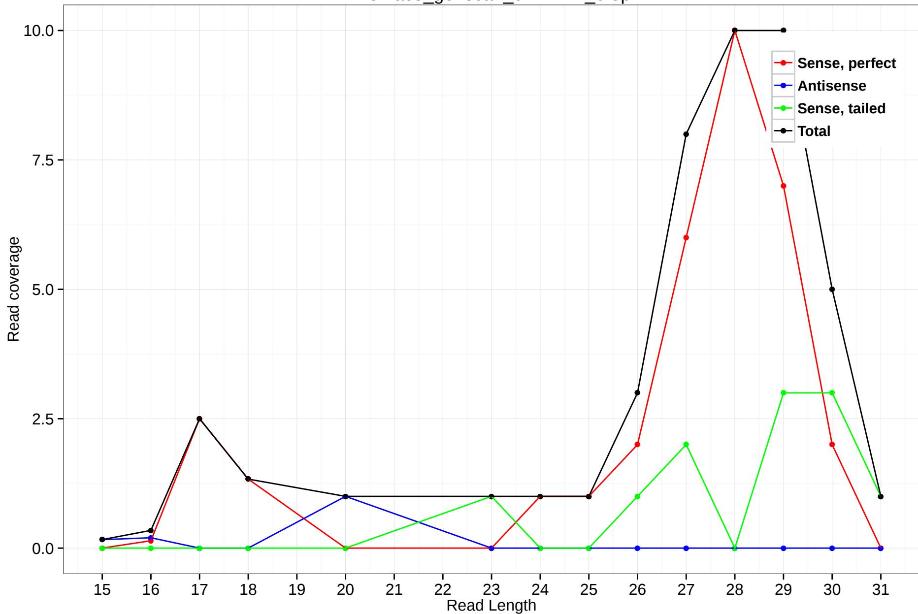
rheMac3_genscan_chr11.22_0.5p
