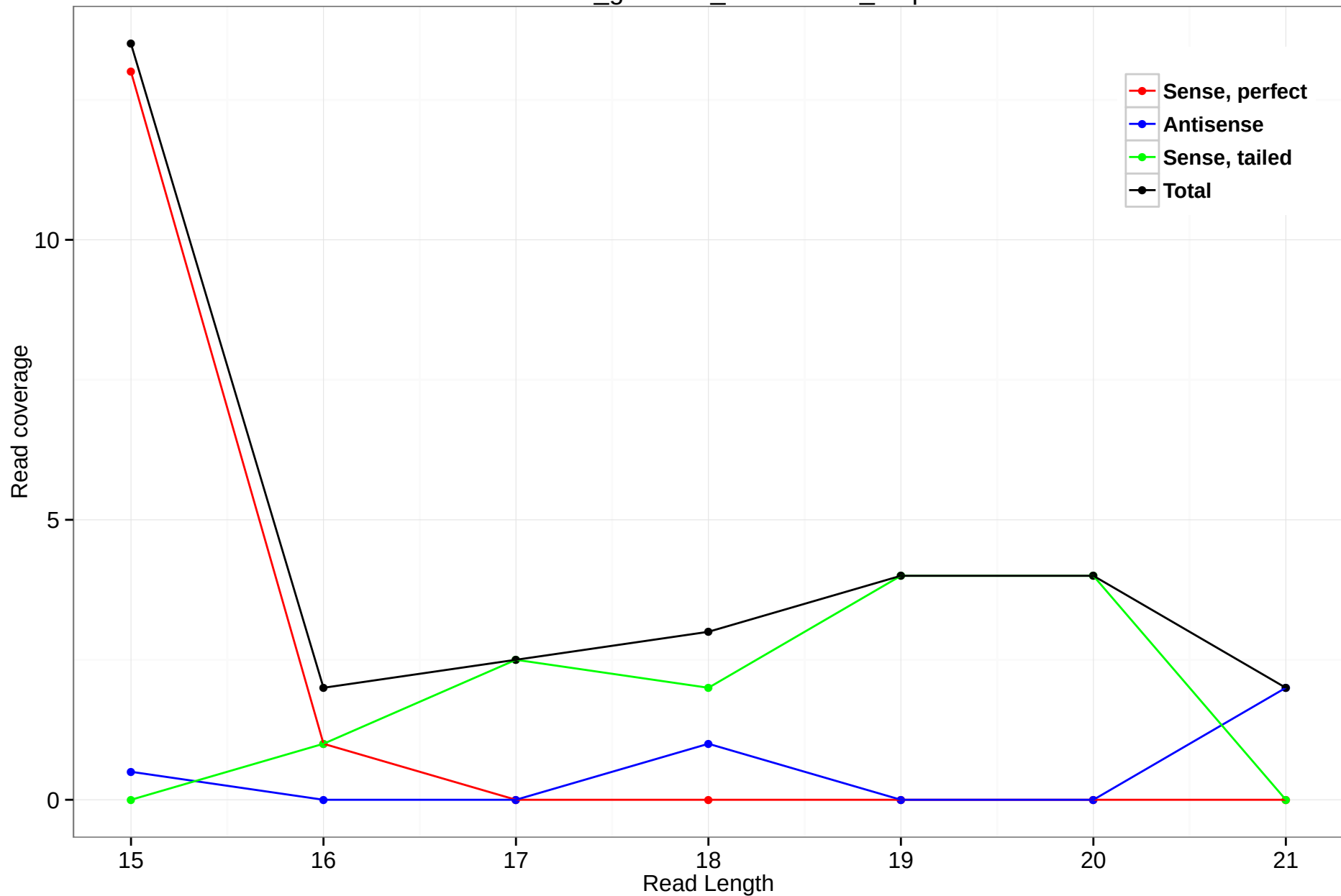
rheMac3_genscan_chr11.2291_0.5p
