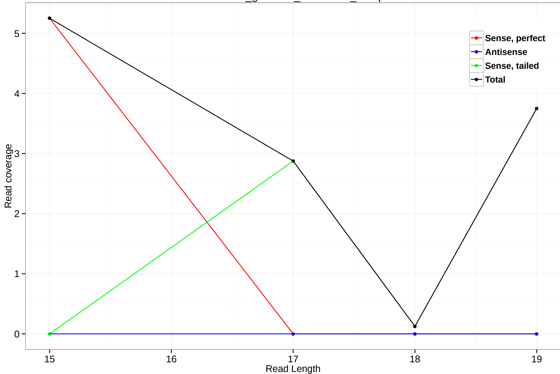
rheMac3_genscan_chr11.227_20.5p
