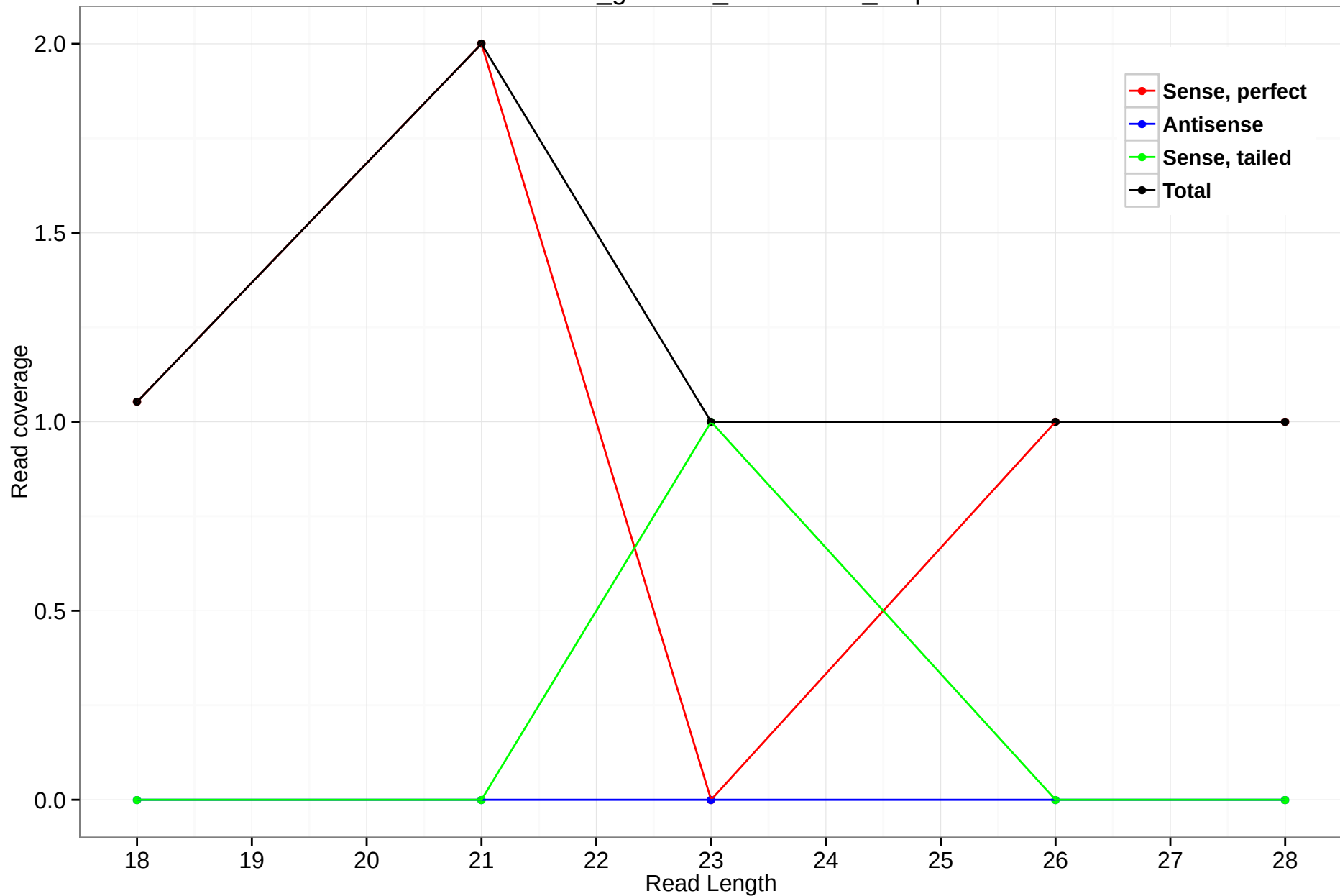
rheMac3_genscan_chr11.2277_2.3p
