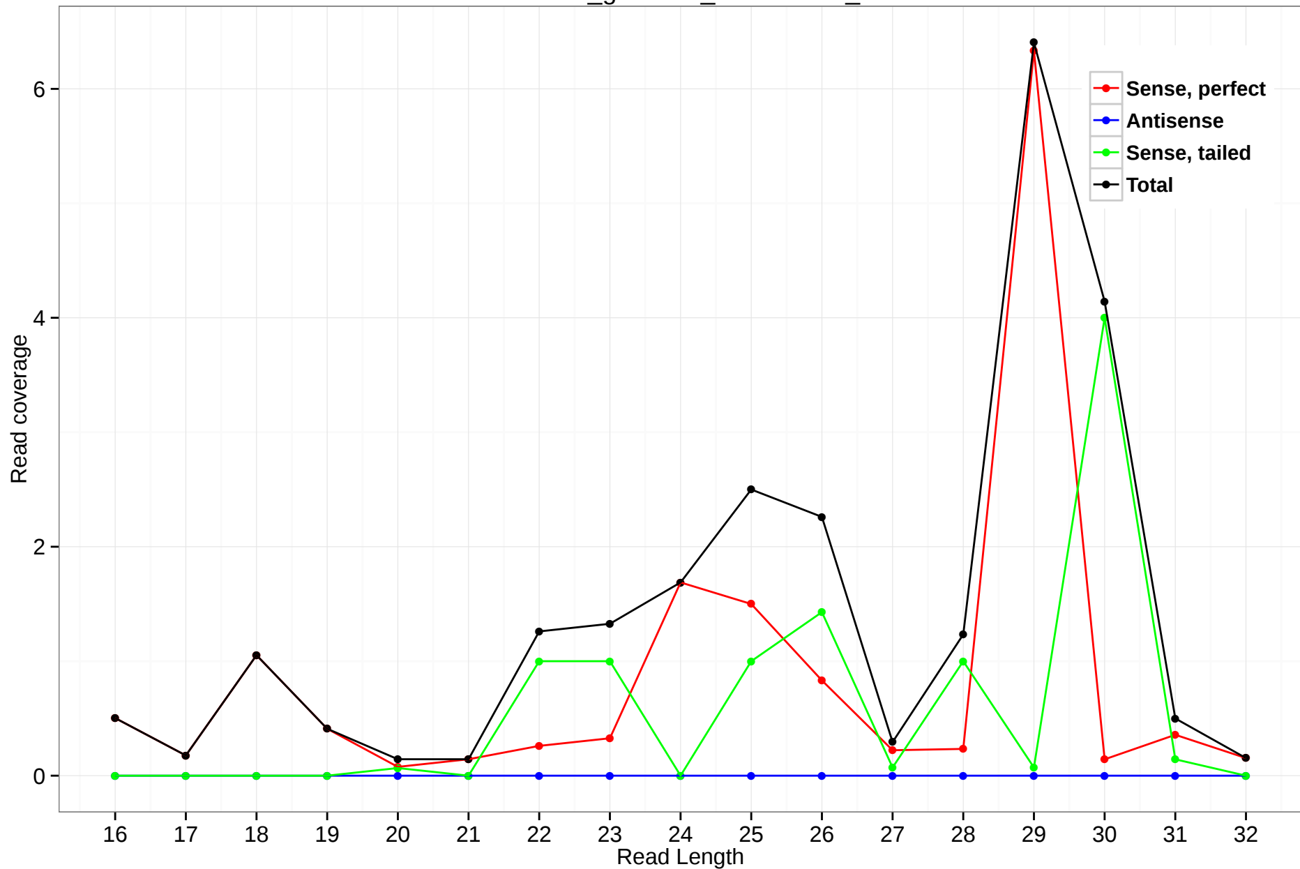
rheMac3_genscan_chr11.2261_1
