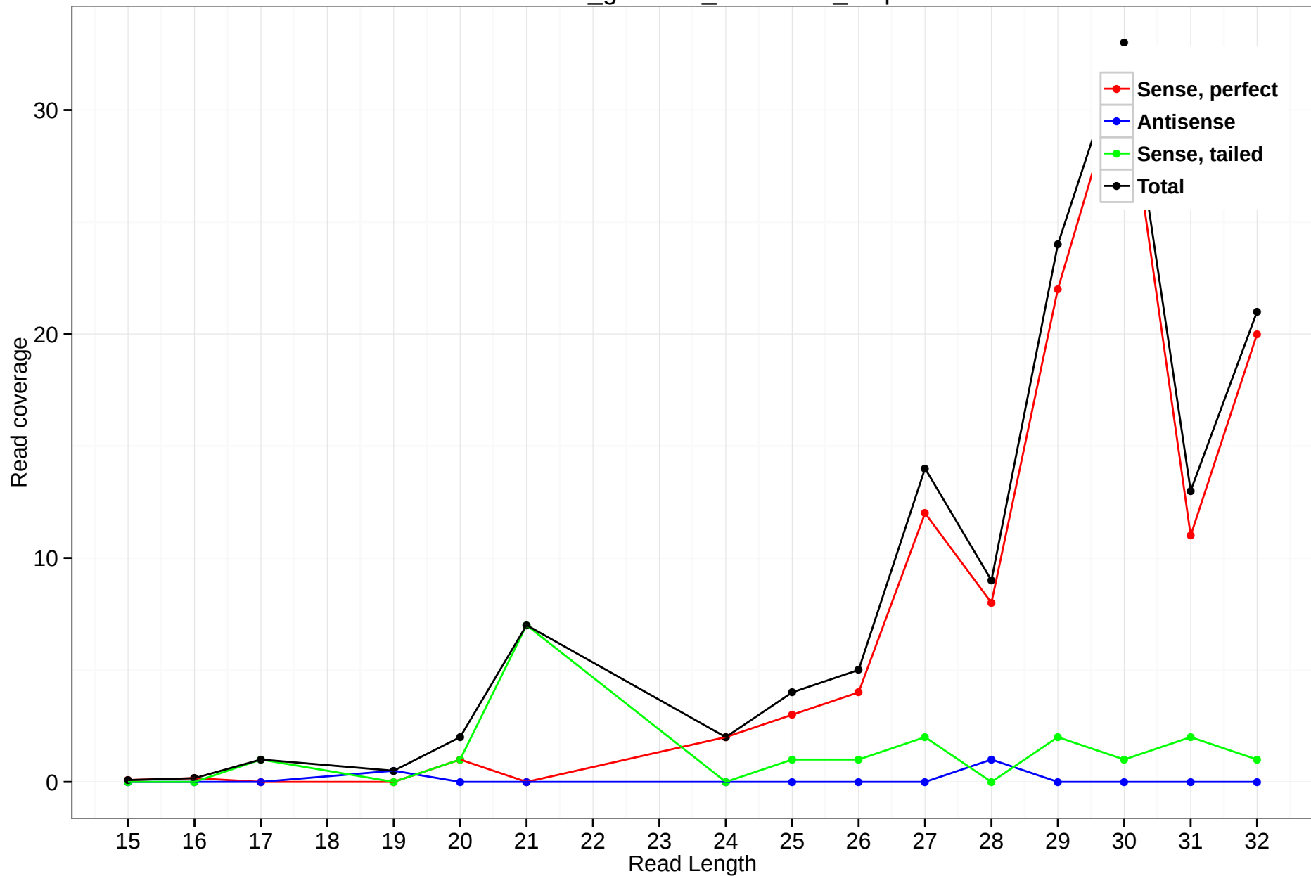
rheMac3_genscan_chr11.225_9.5p
