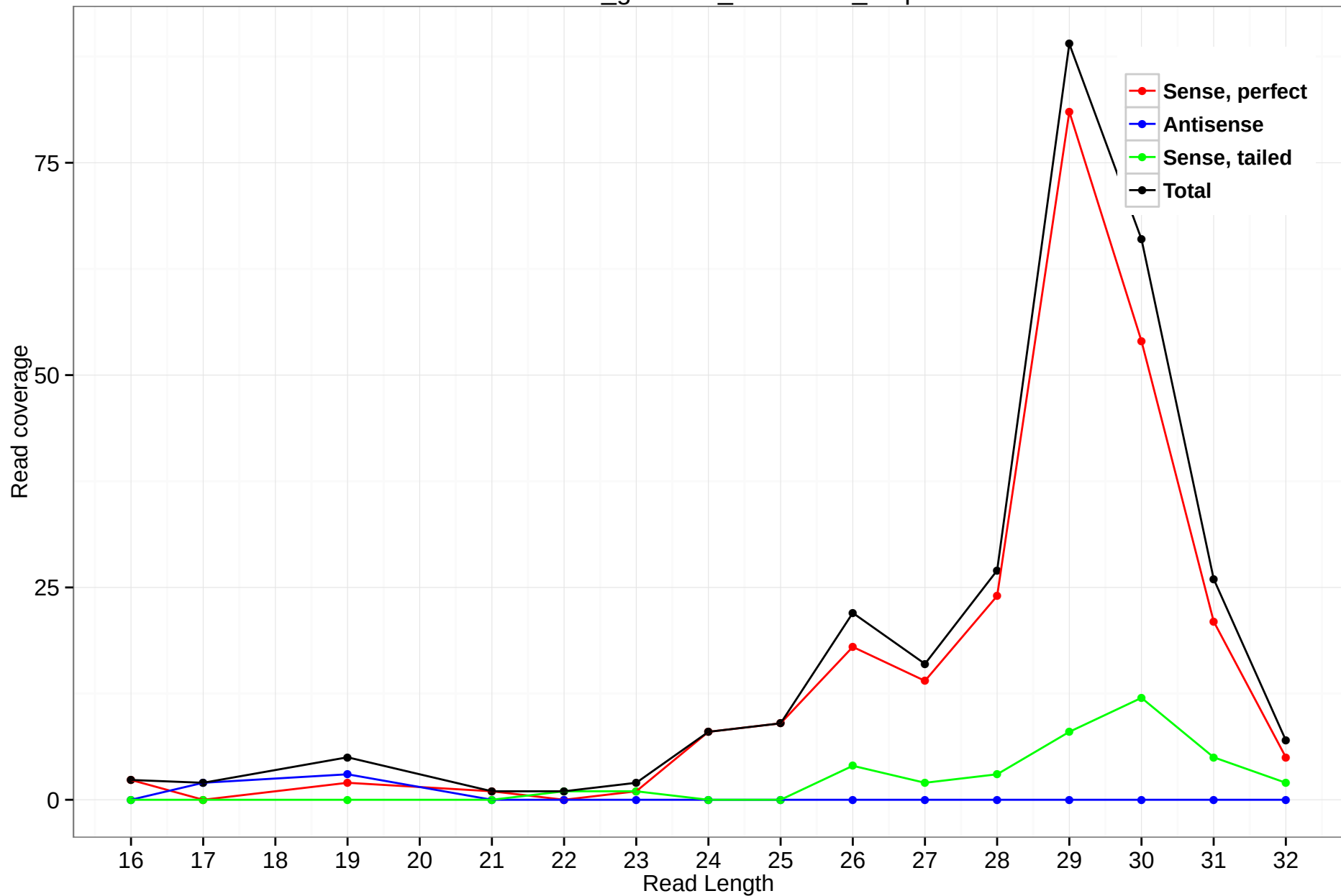
rheMac3_genscan_chr11.225_9.3p
