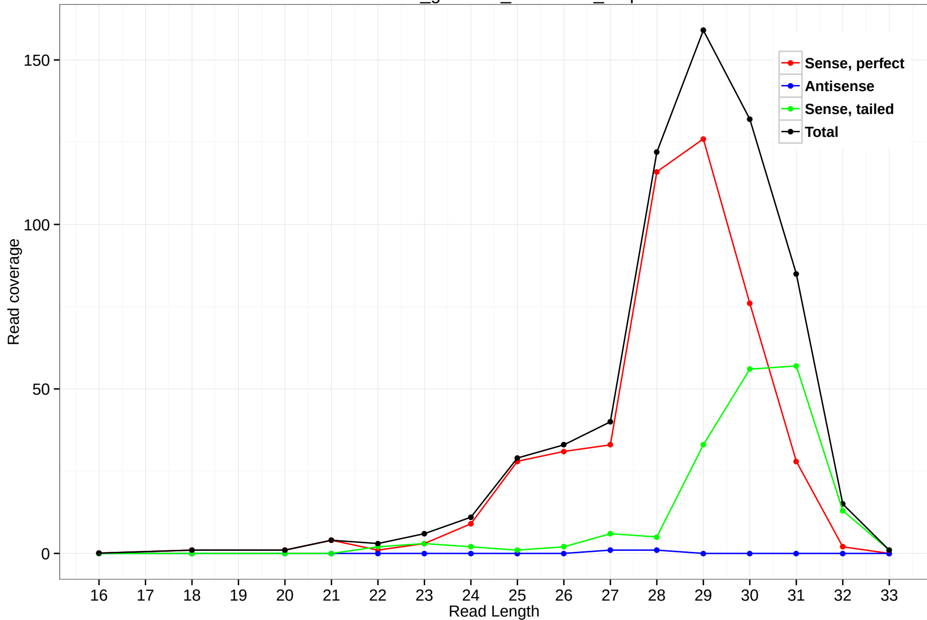
rheMac3_genscan_chr11.225_7.5p
