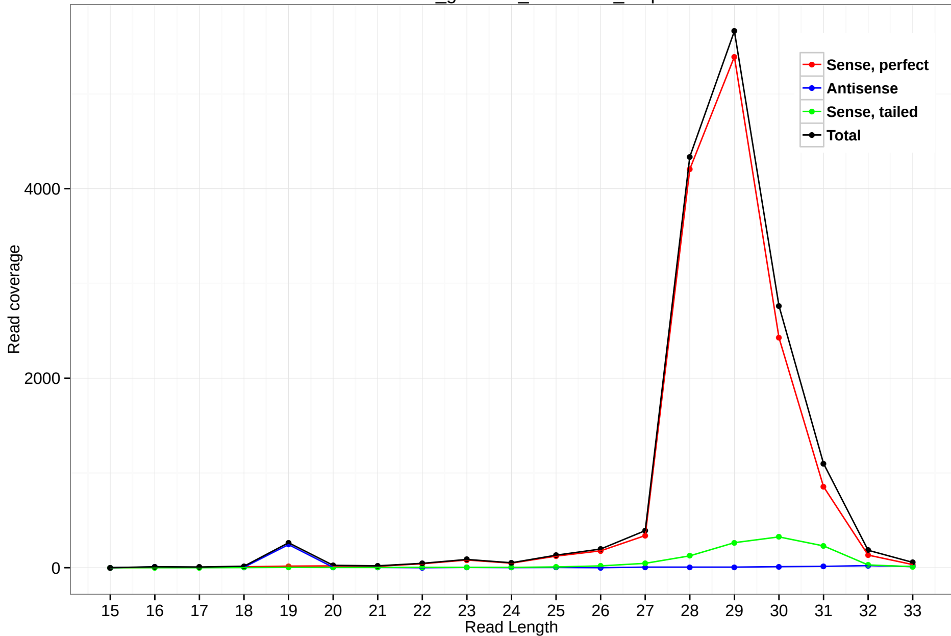
rheMac3_genscan_chr11.225_5.5p
