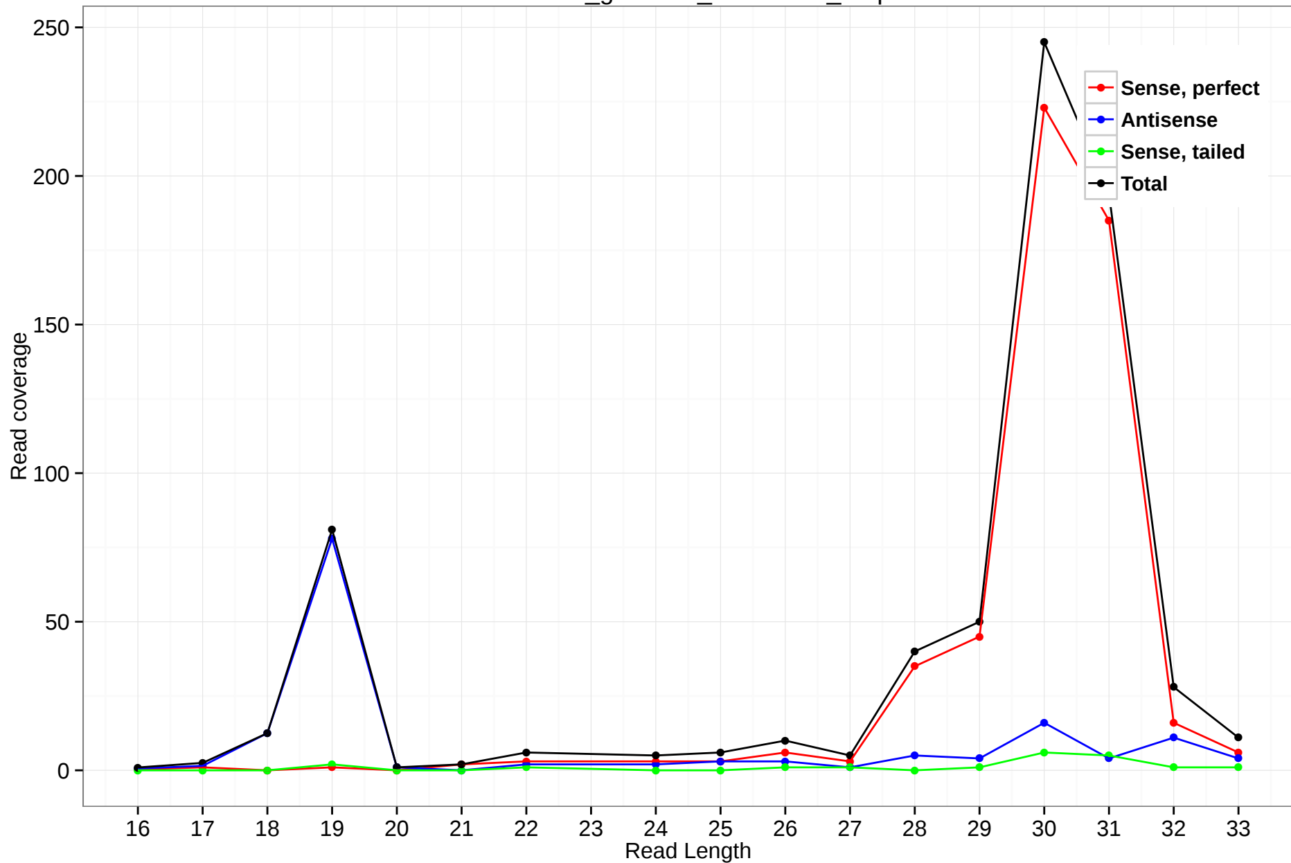
rheMac3_genscan_chr11.225_3.3p
