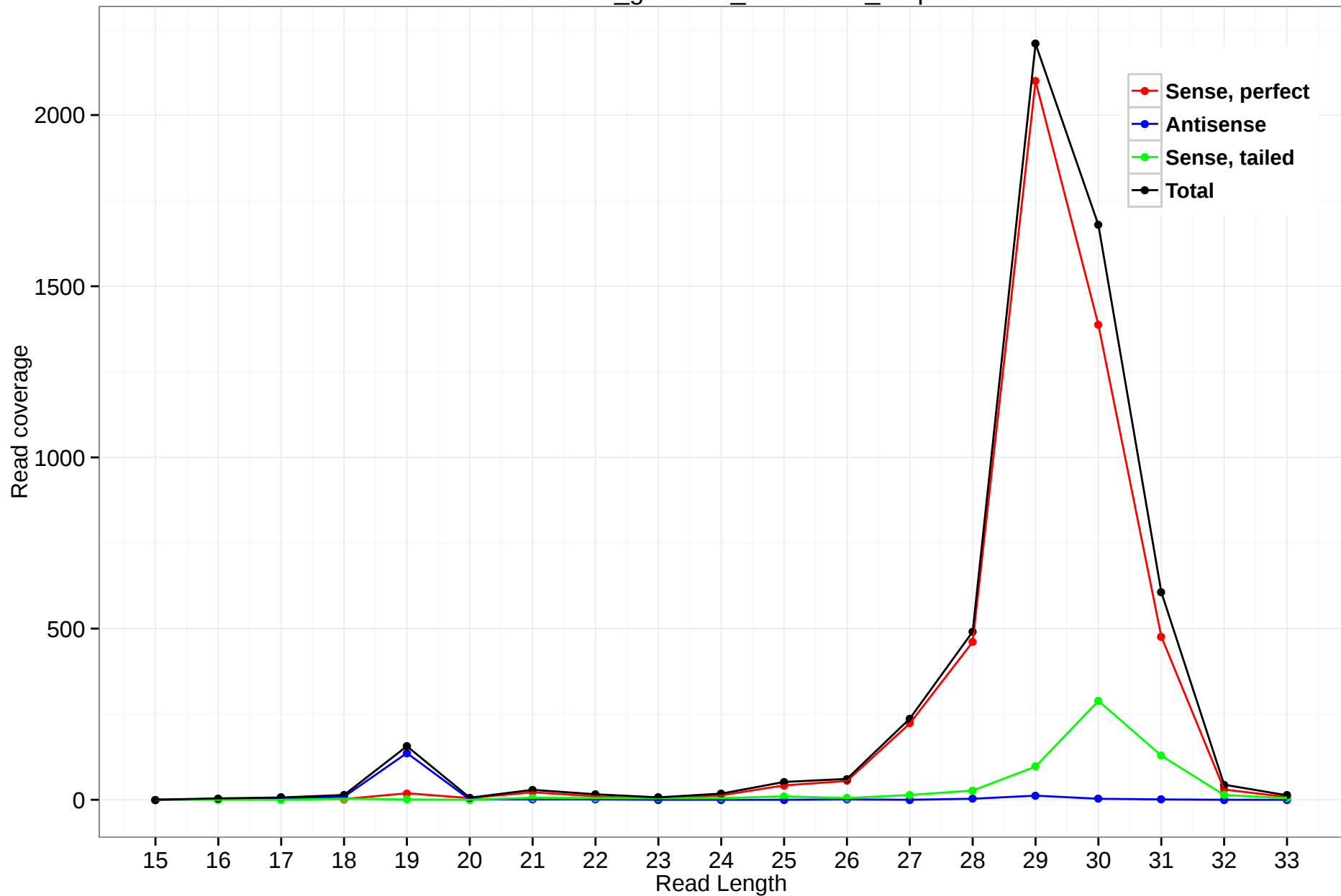
rheMac3_genscan_chr11.225_0.5p
