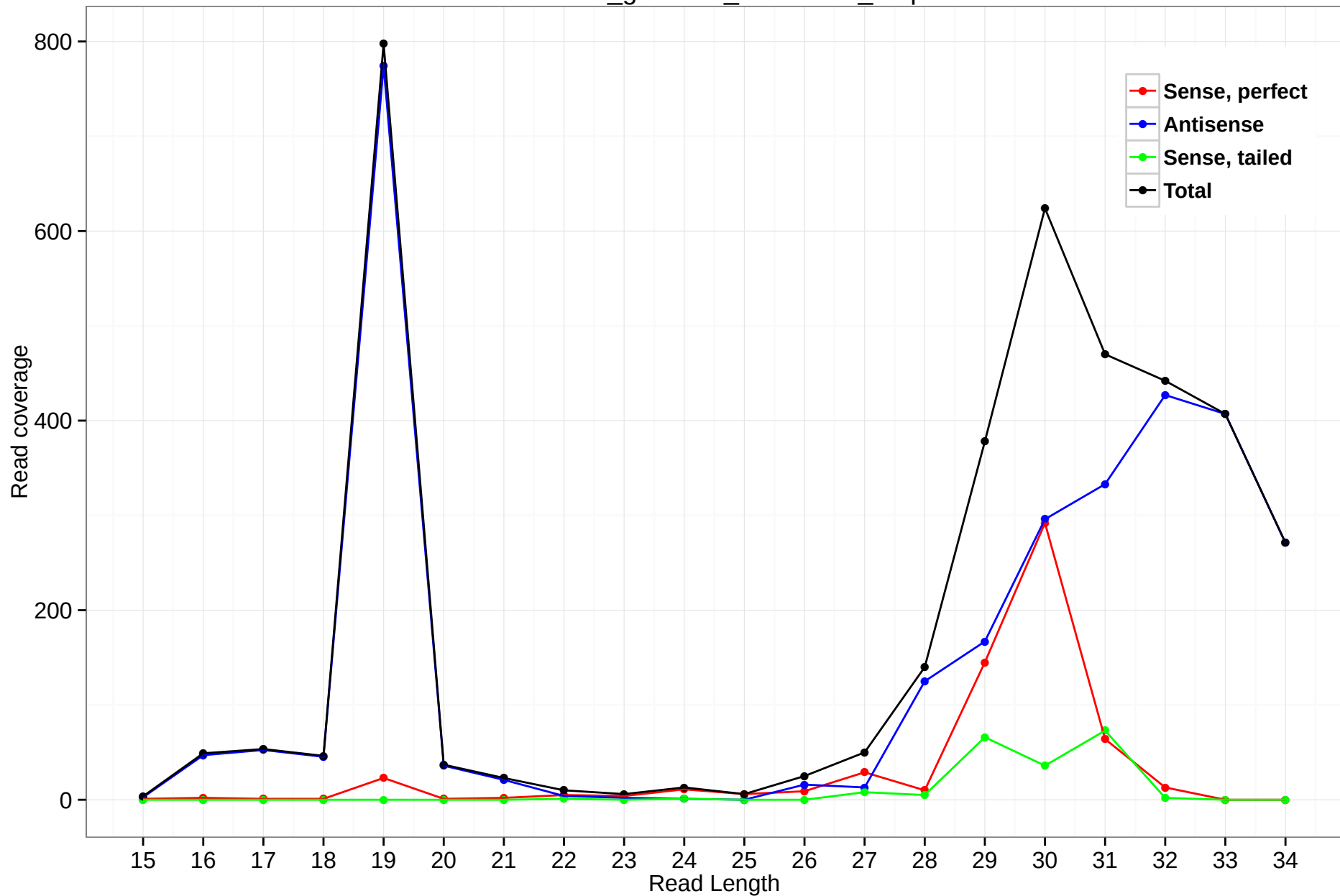
rheMac3_genscan_chr11.225_0.3p
