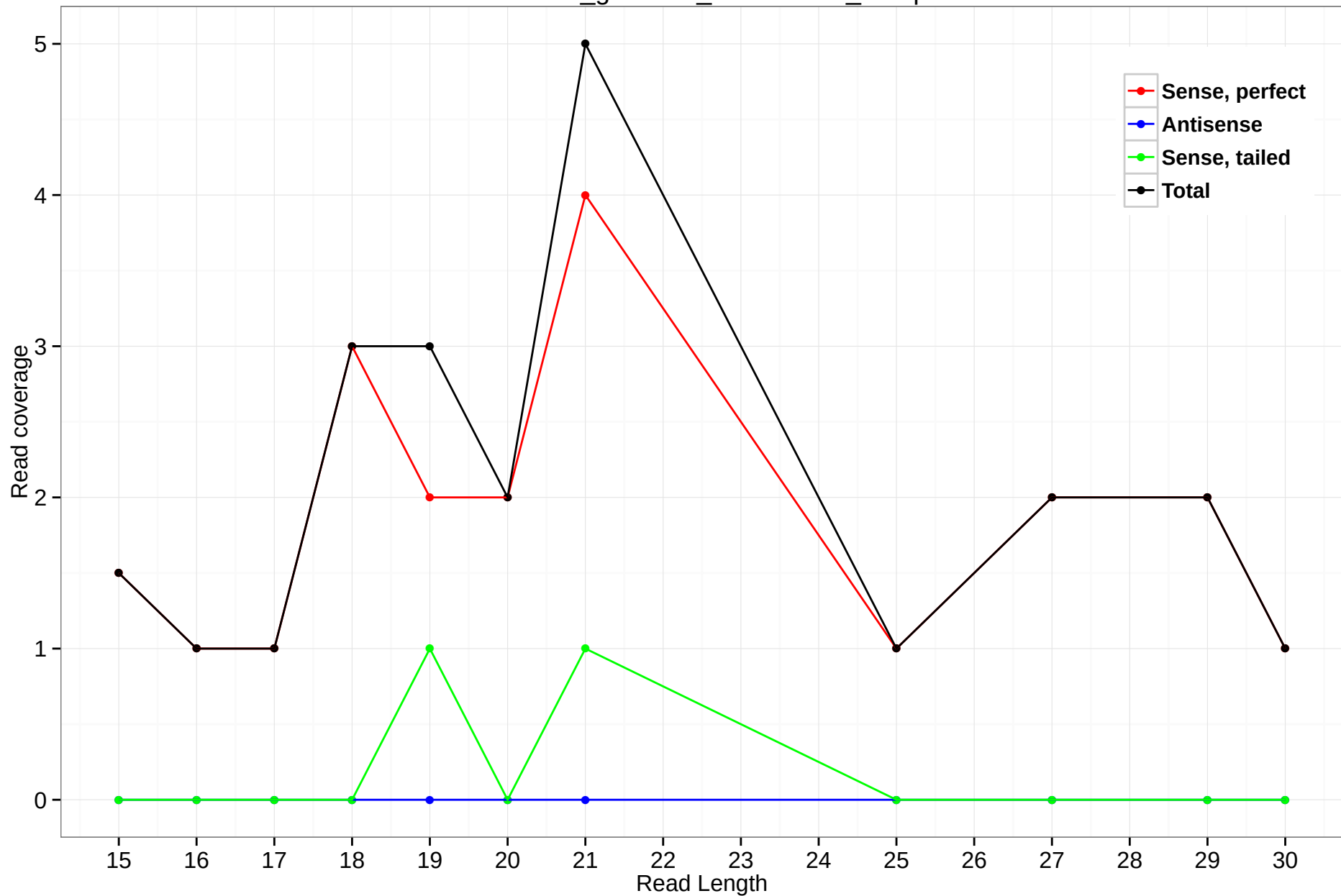
rheMac3_genscan_chr11.2235_20.3p
