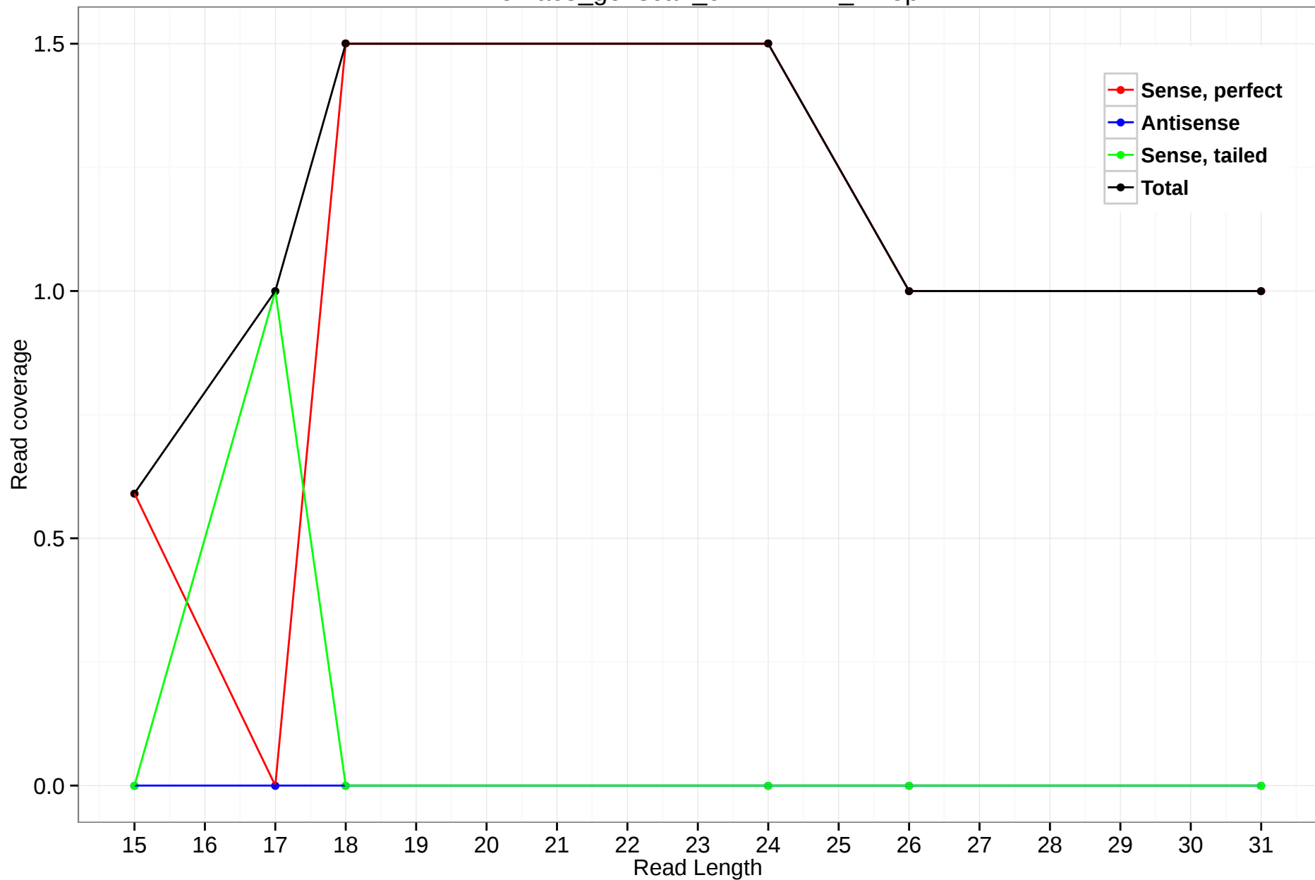
rheMac3_genscan_chr11.2212_14.5p
